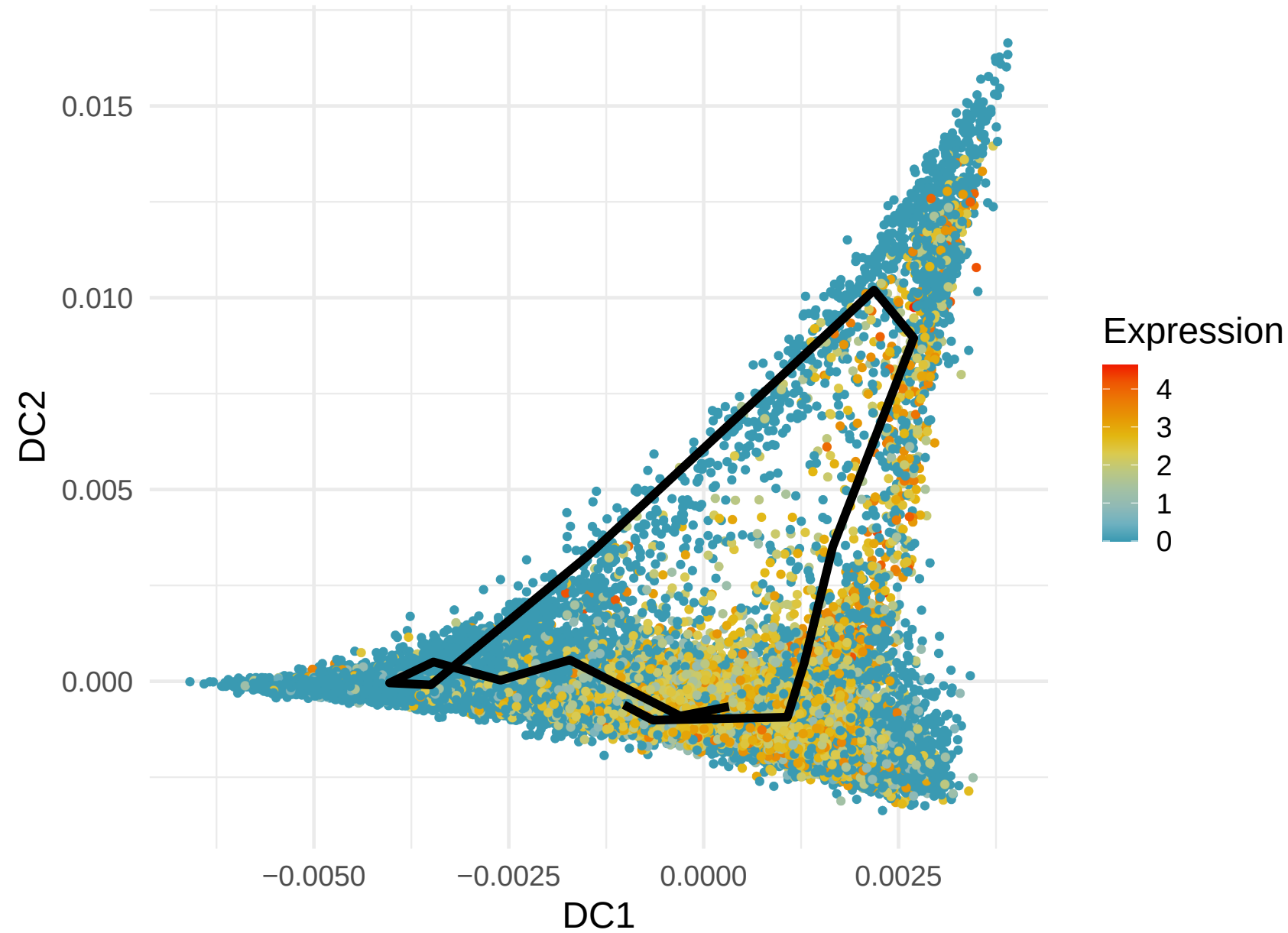
GZMK Expression along Lineage 3 (R= 0.319)
