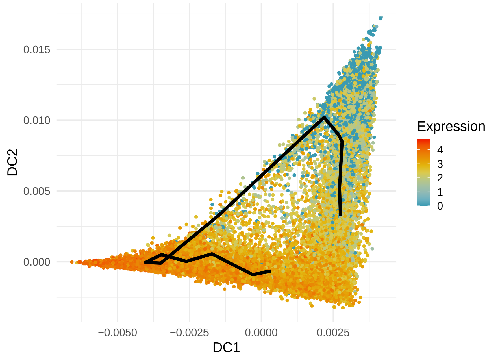
RPS13 Expression along Lineage 4 ( R = -0.401 )
