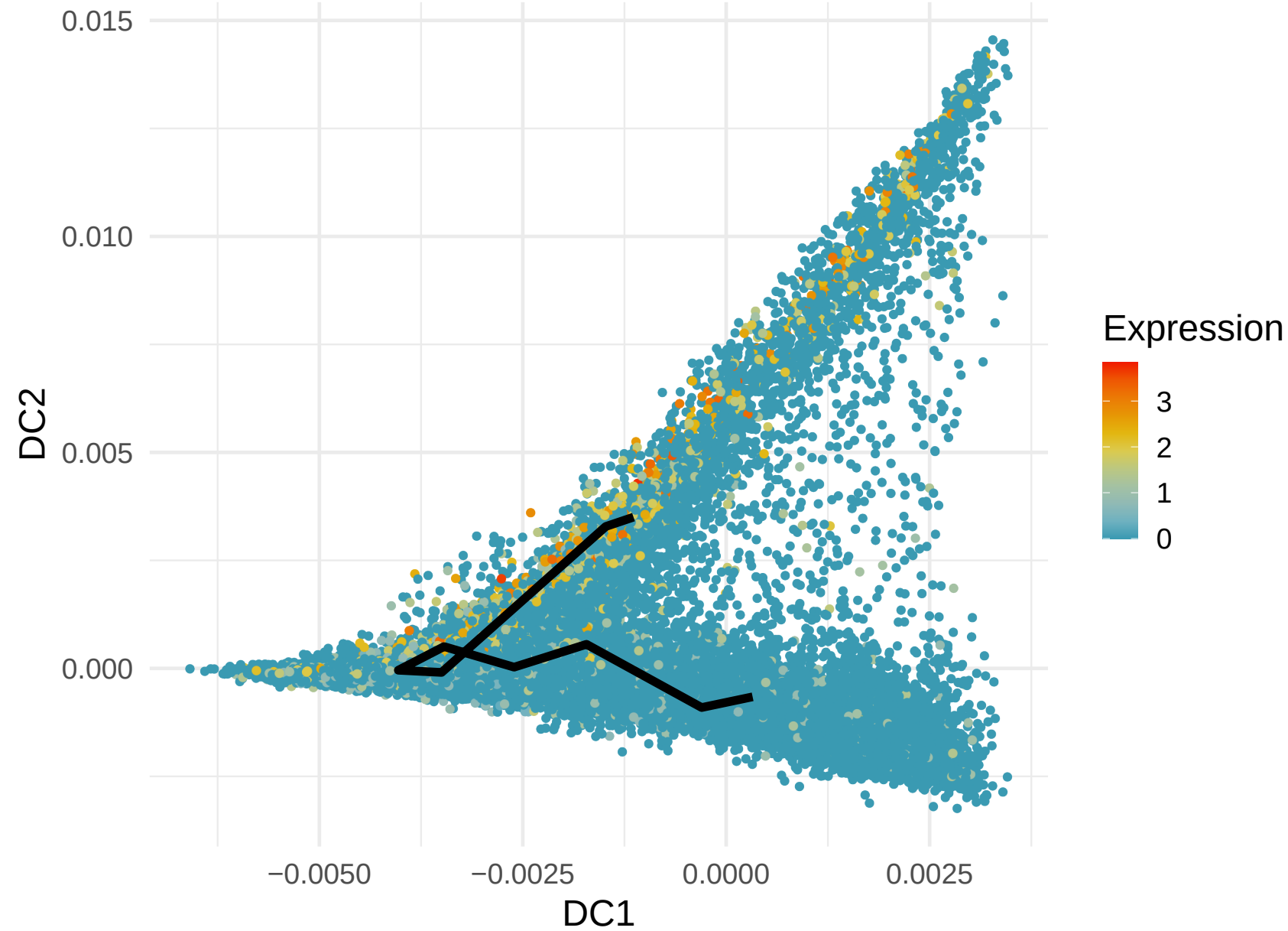
FAM13A Expression along Lineage 5 ( R = 0.245 )
