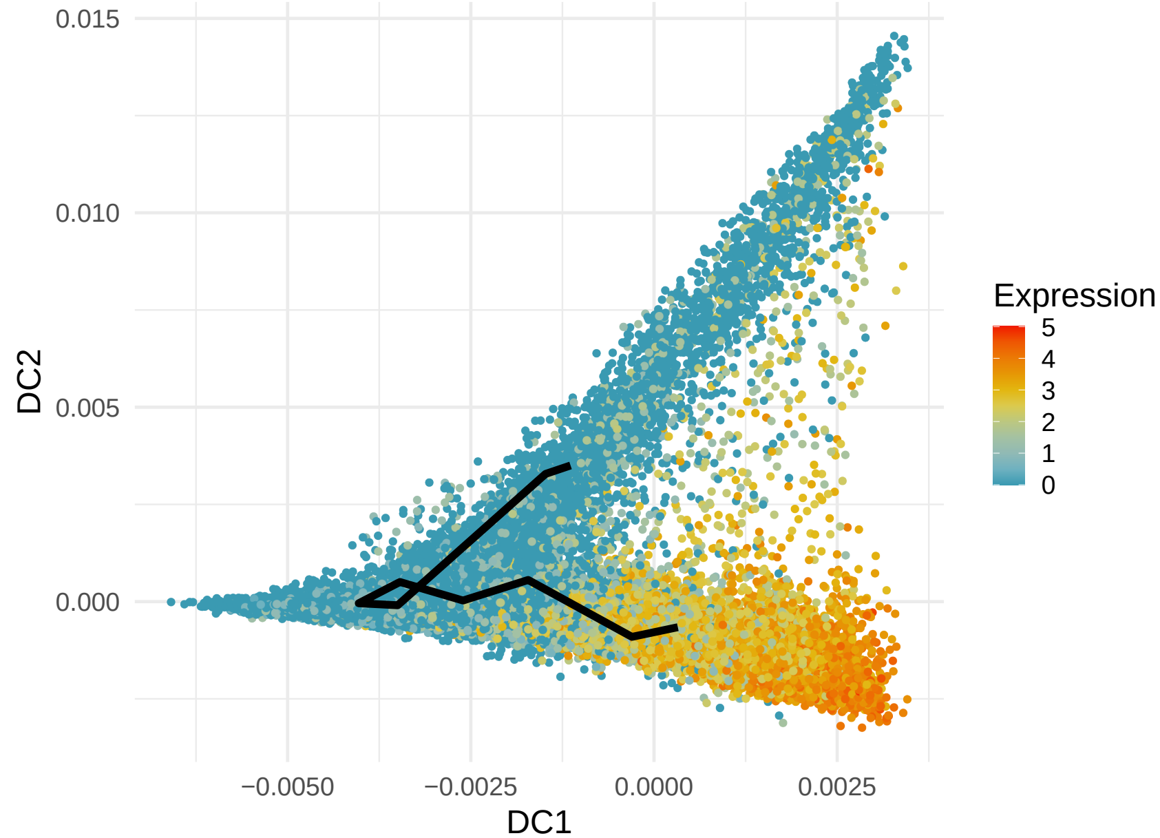
NKG7 Expression along Lineage 5 ( R = -0.488 )
