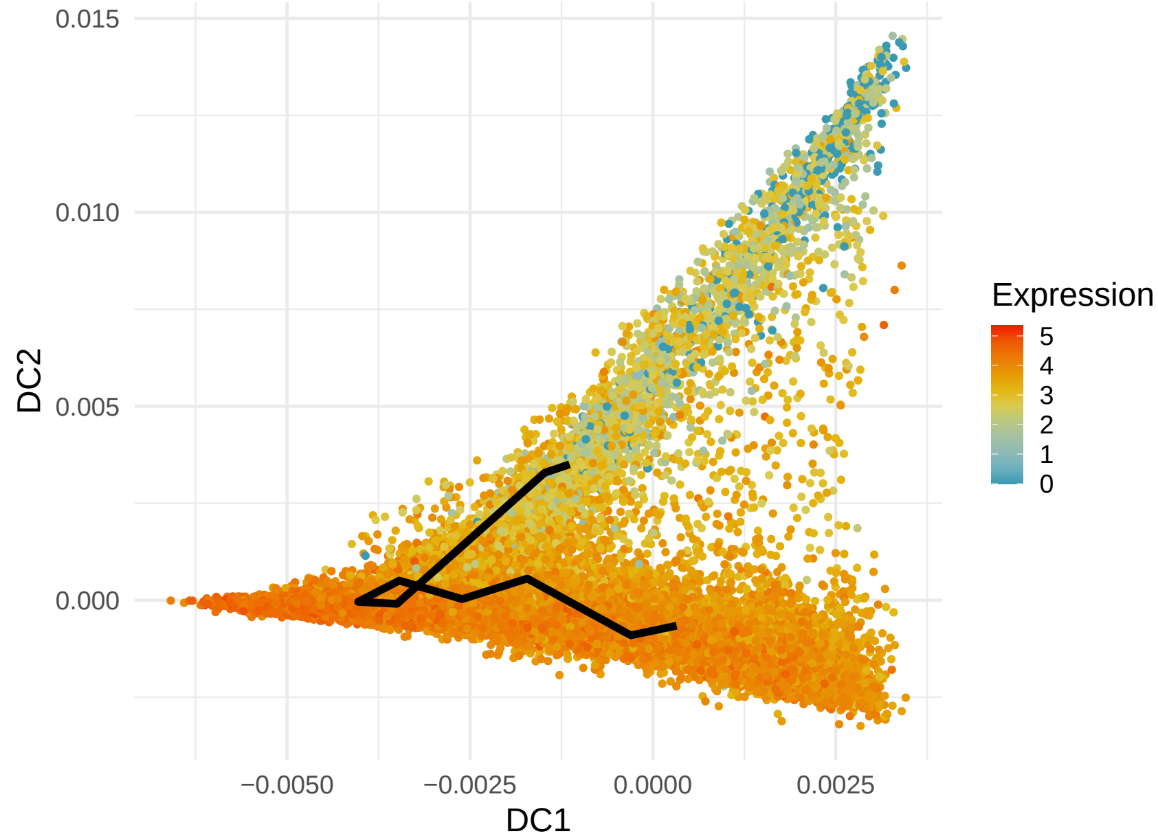
RPS27A Expression along Lineage 5 ( R = -0.437 )
