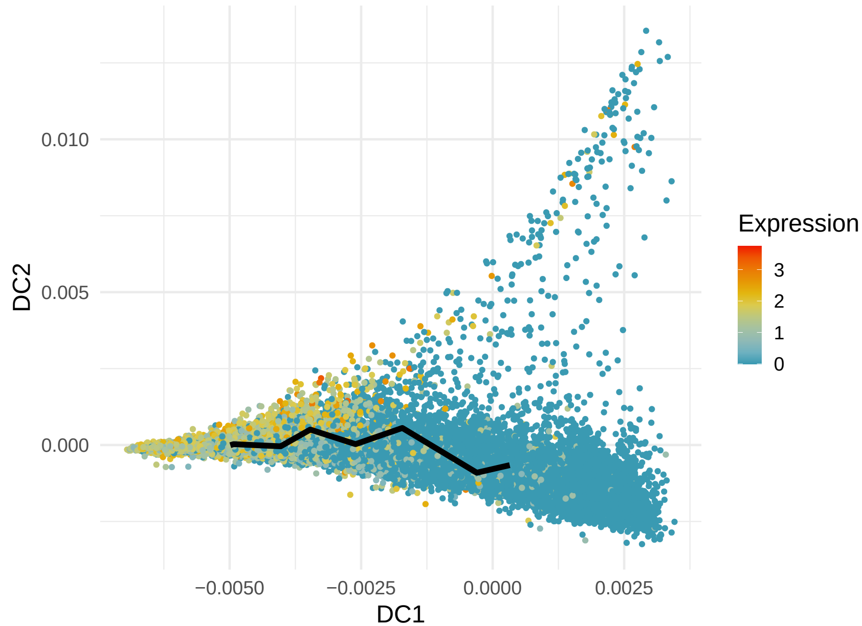
CCR7 Expression along Lineage 6 ( R = 0.58 )
