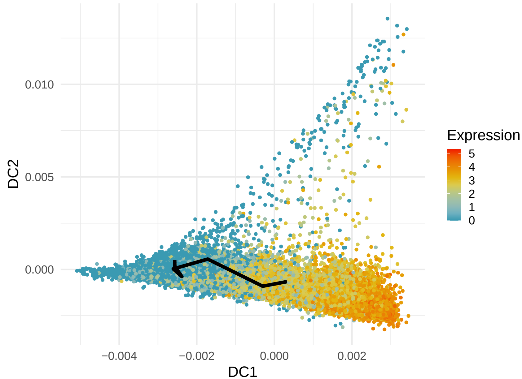
NKG7 Expression along Lineage 7 ( R = -0.58 )
