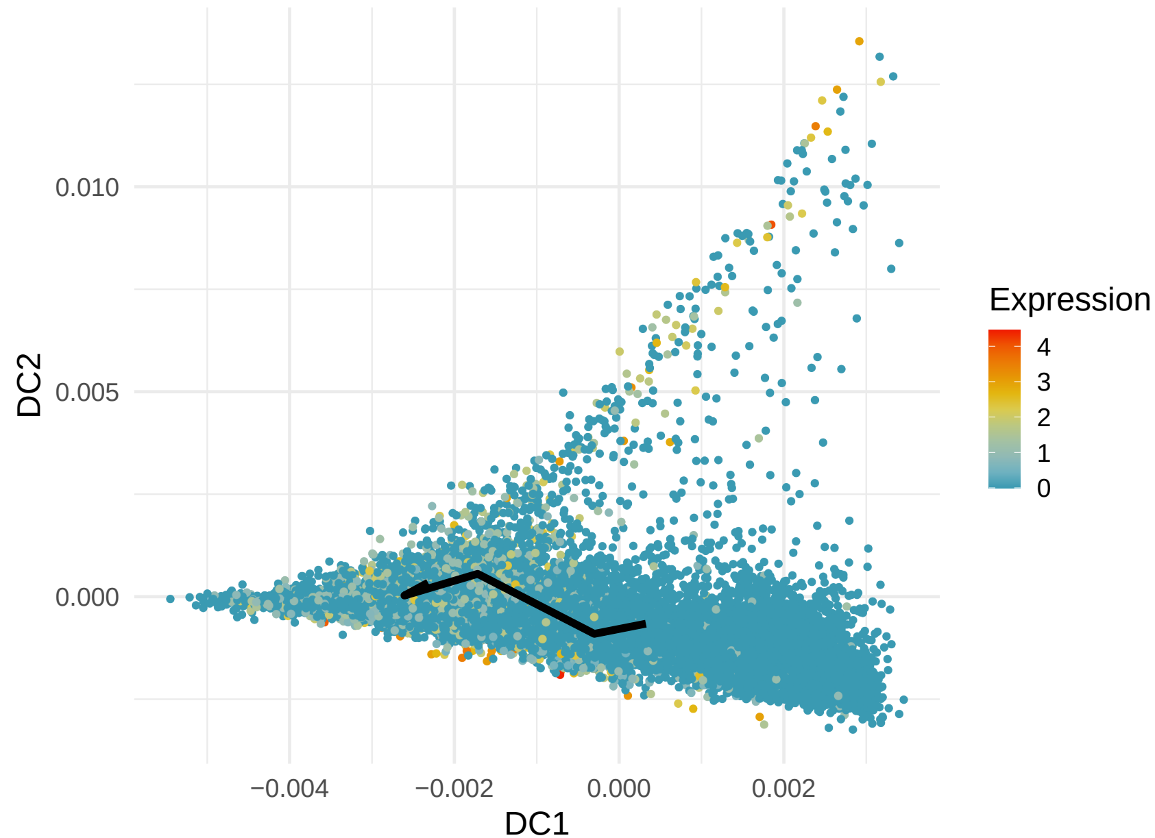
TNFRSF4 Expression along Lineage 8 ( R = 0.345 )
