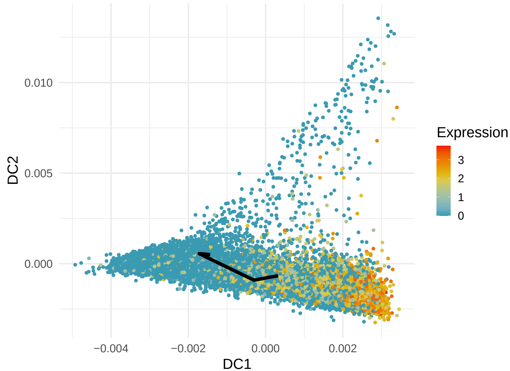
KLRD1 Expression along Lineage 9 ( R = -0.409 )
