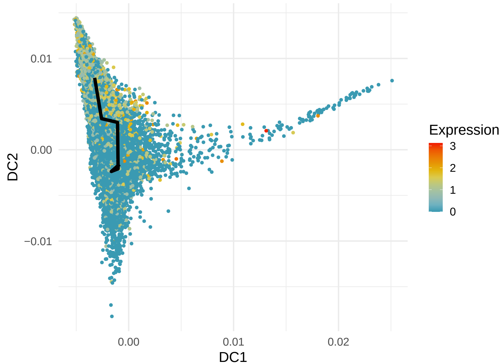
AlF1 Expression along Lineage 1 ( R = -0.313 )
