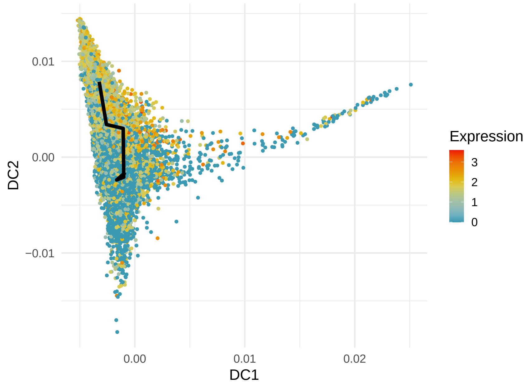
SELL Expression along Lineage 1 ( R = -0.364 )
