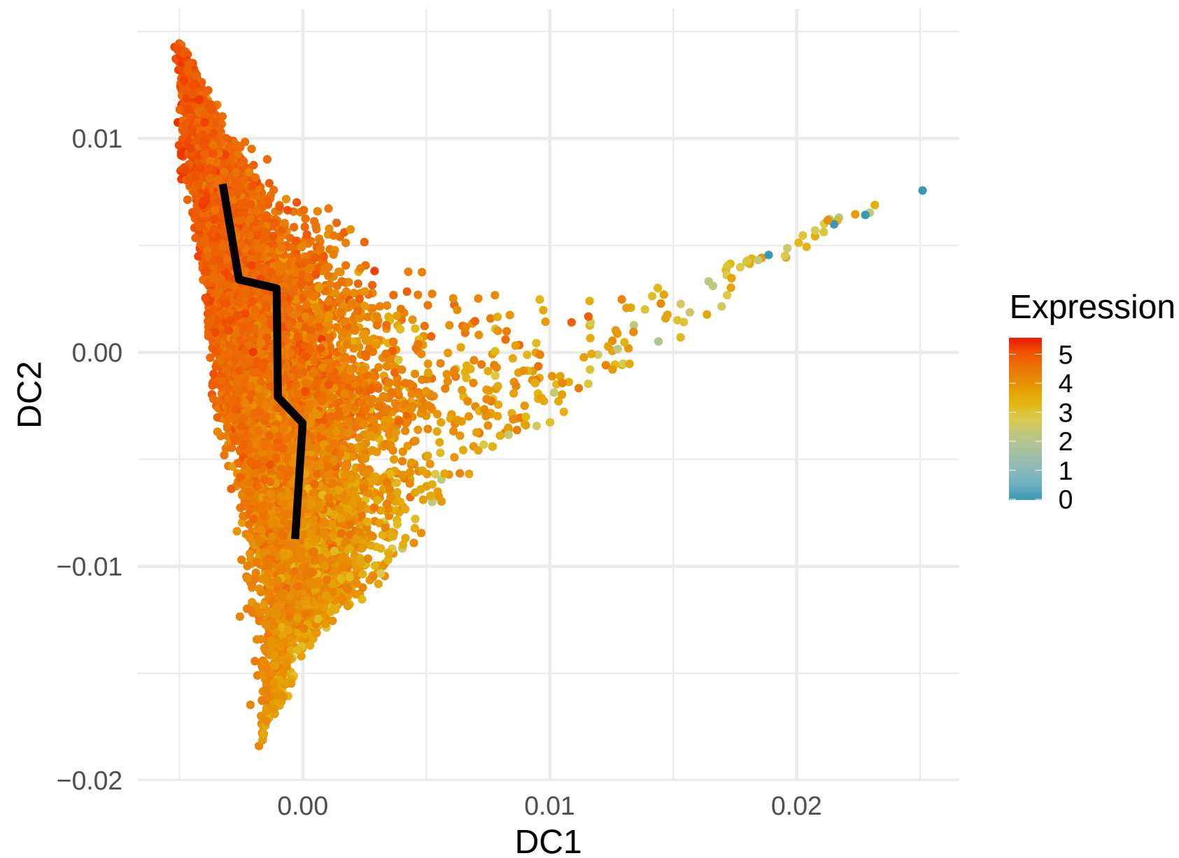
RPL13 Expression along Lineage 2 ( R = -0.49 )
