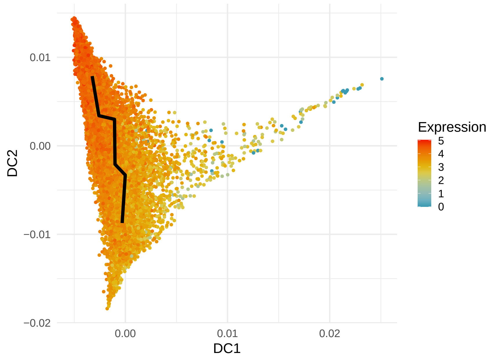
RPS3A Expression along Lineage 2 ( R = -0.45 )
