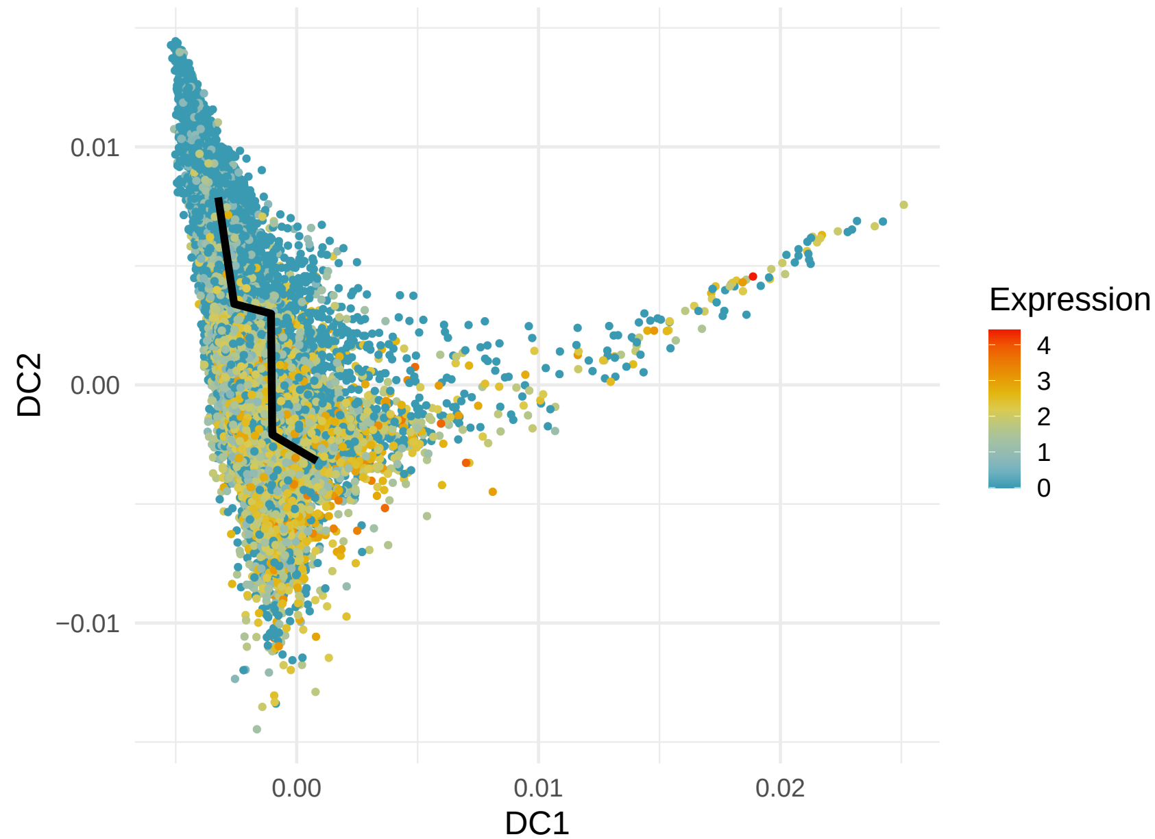
ITGB1 Expression along Lineage 3 (R= 0.328)
