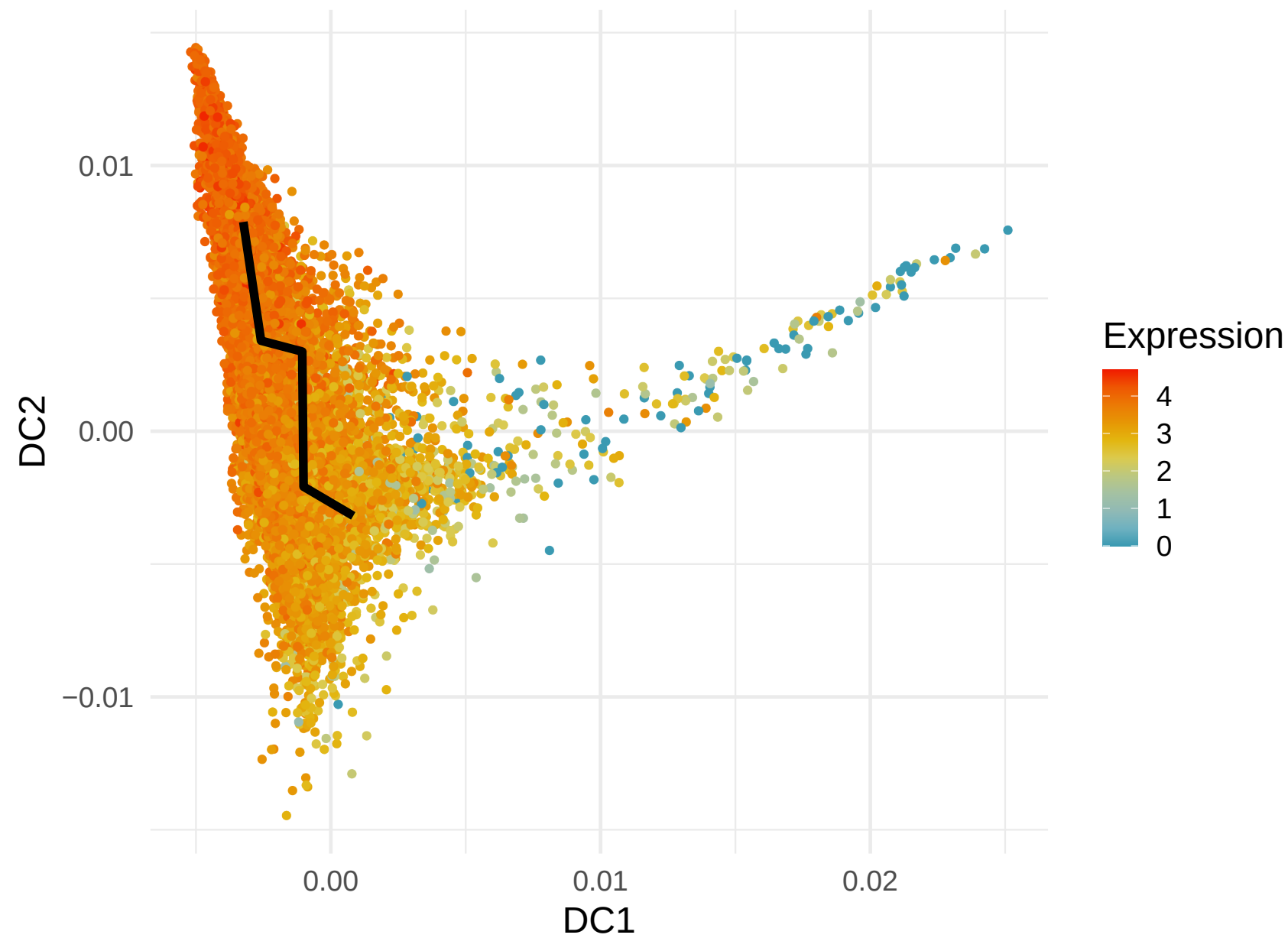
RPS13 Expression along Lineage 3 ( R = -0.478 )
