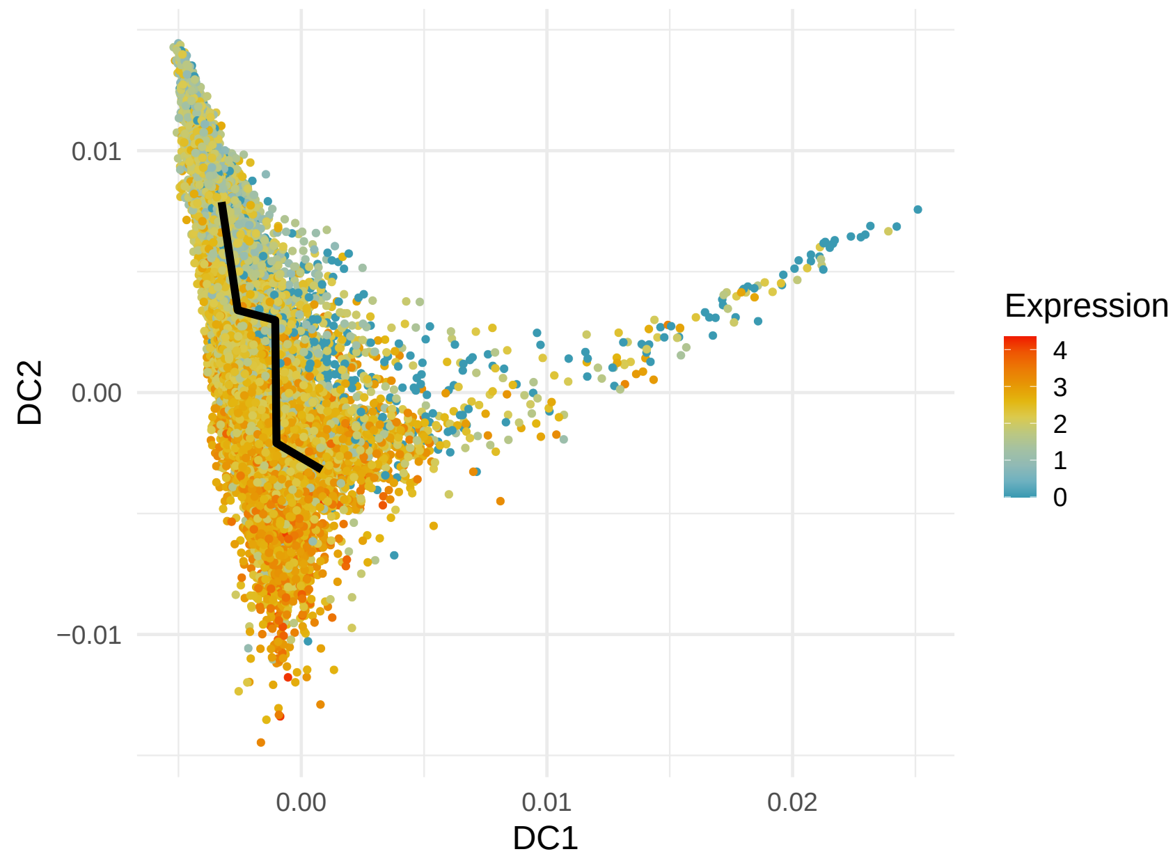
SH3BGRL3 Expression along Lineage 3 ( R = 0.366 )
