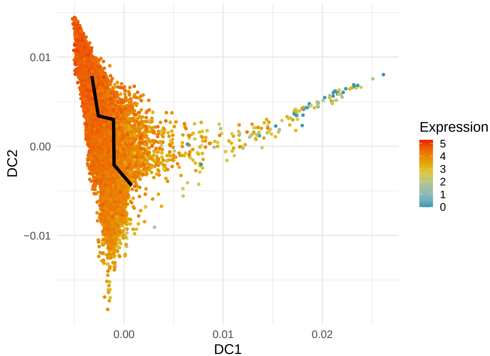
RPL30 Expression along Lineage 4 ( R = -0.429 )
