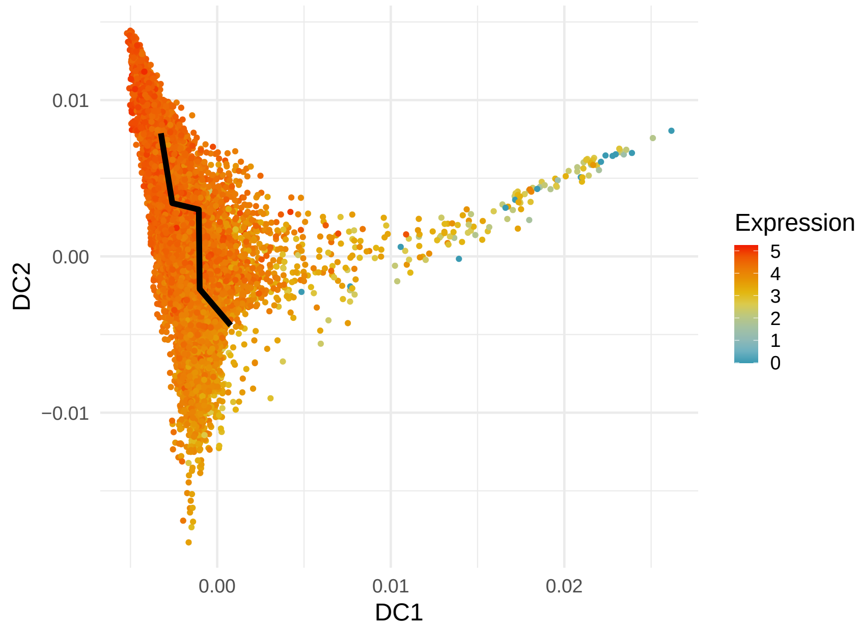
RPL32 Expression along Lineage 4 ( R = -0.484 )
