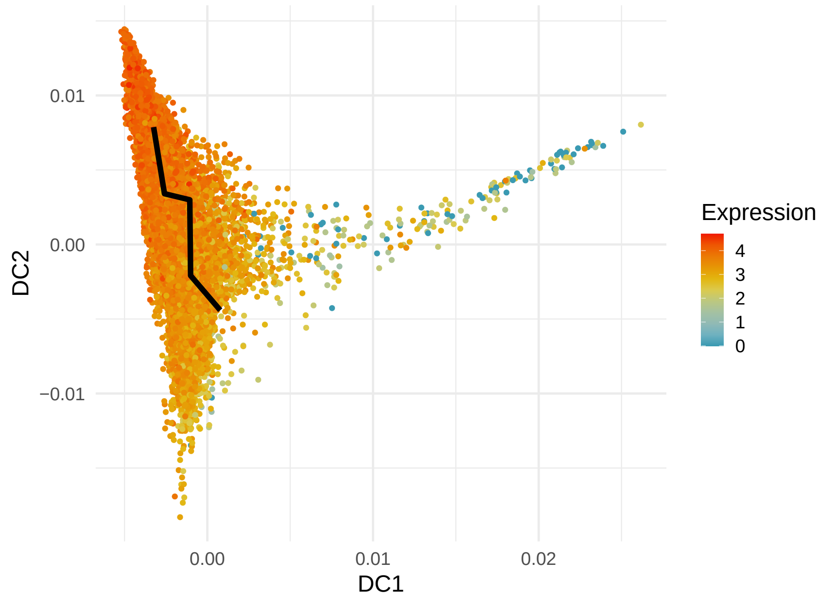
RPS13 Expression along Lineage 4 ( R = -0.439 )
