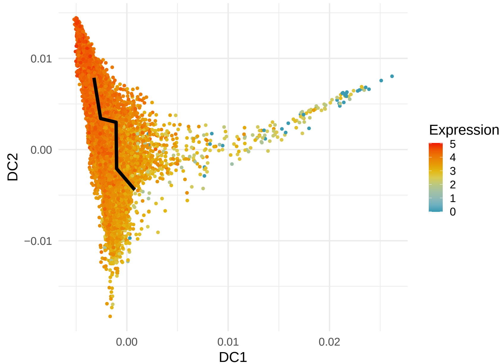
RPS3A Expression along Lineage 4 ( R = -0.48 )
