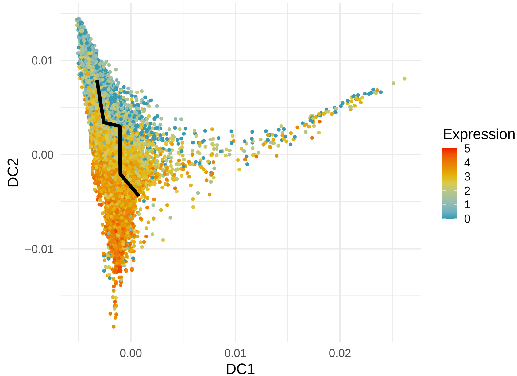
S100A4 Expression along Lineage 4 ( R = 0.589 )
