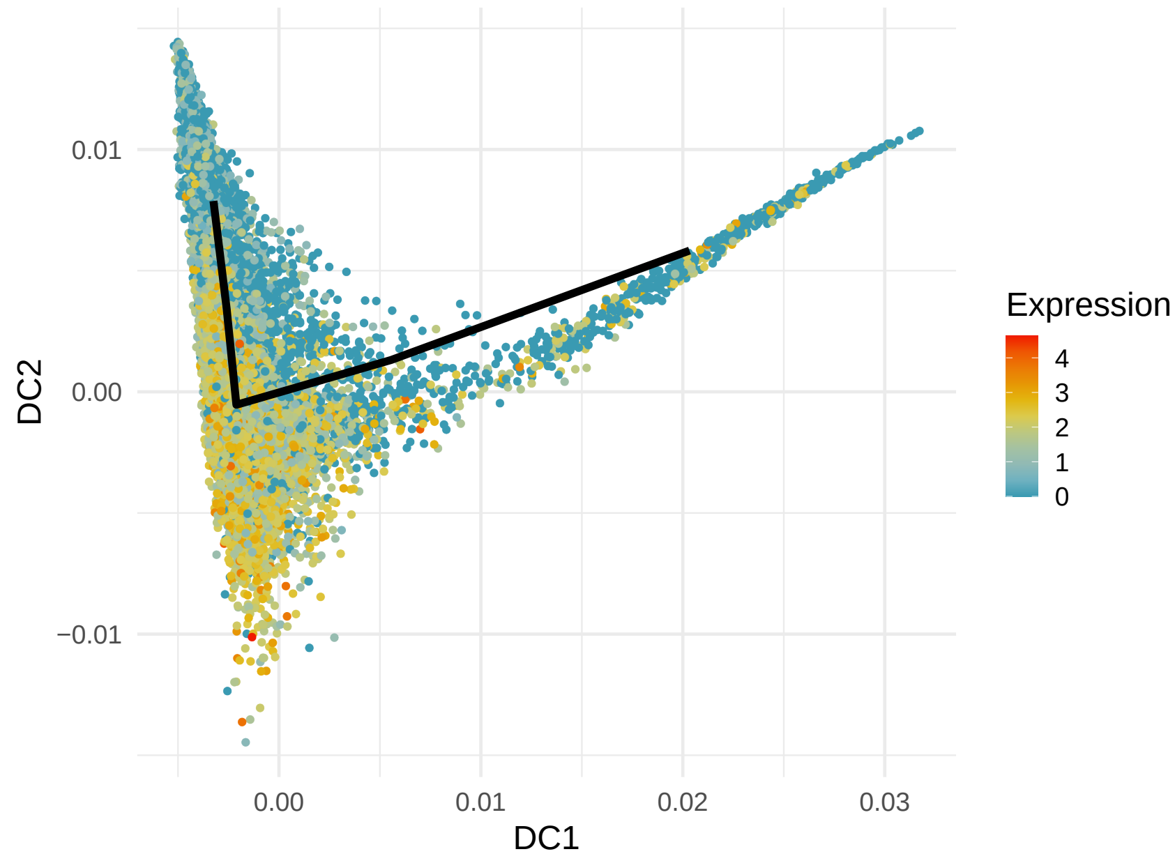
ANXA1 Expression along Lineage 5 ( R = 0.234 )
