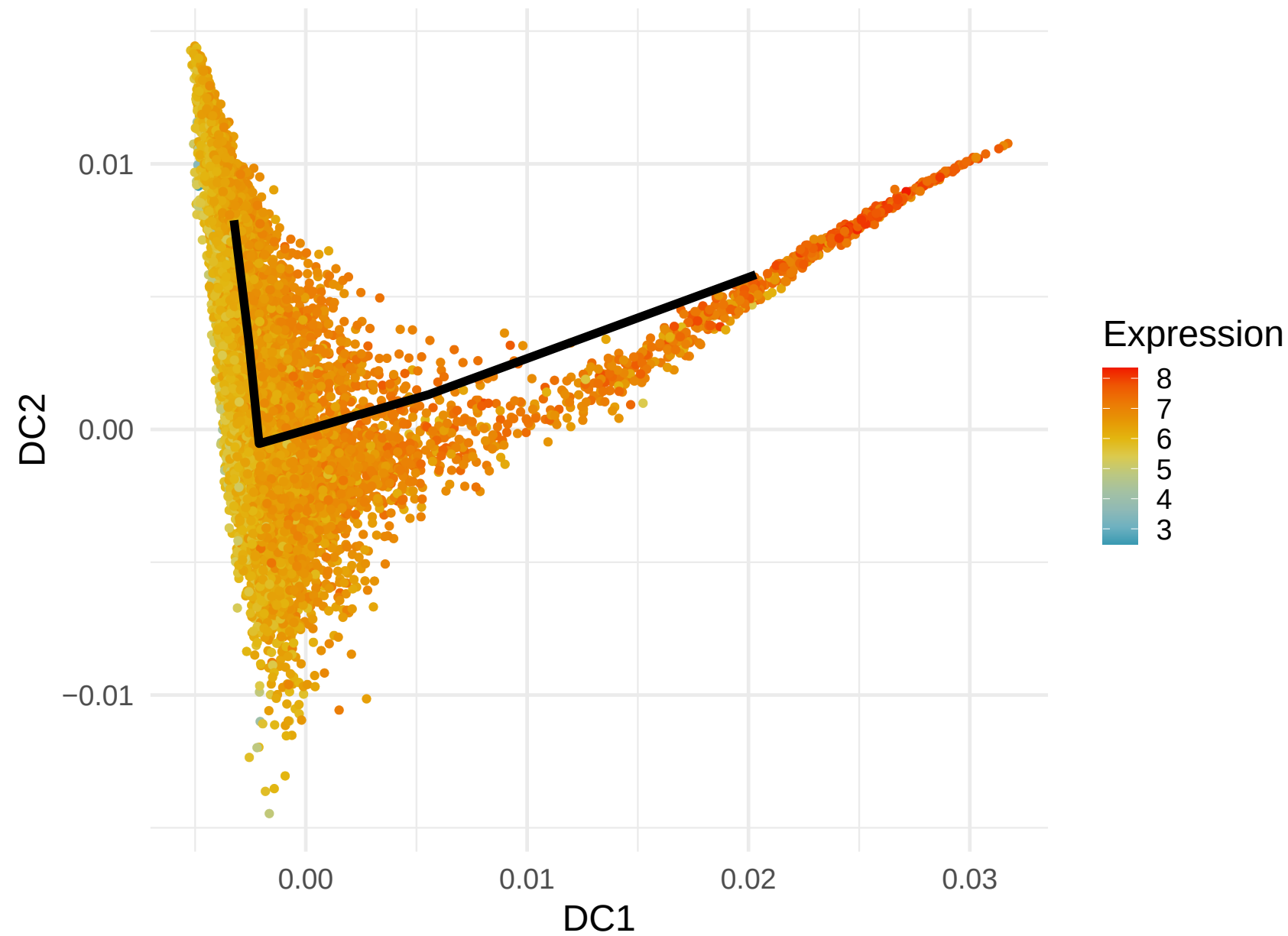
MALAT1 Expression along Lineage 5 ( R = 0.264 )
