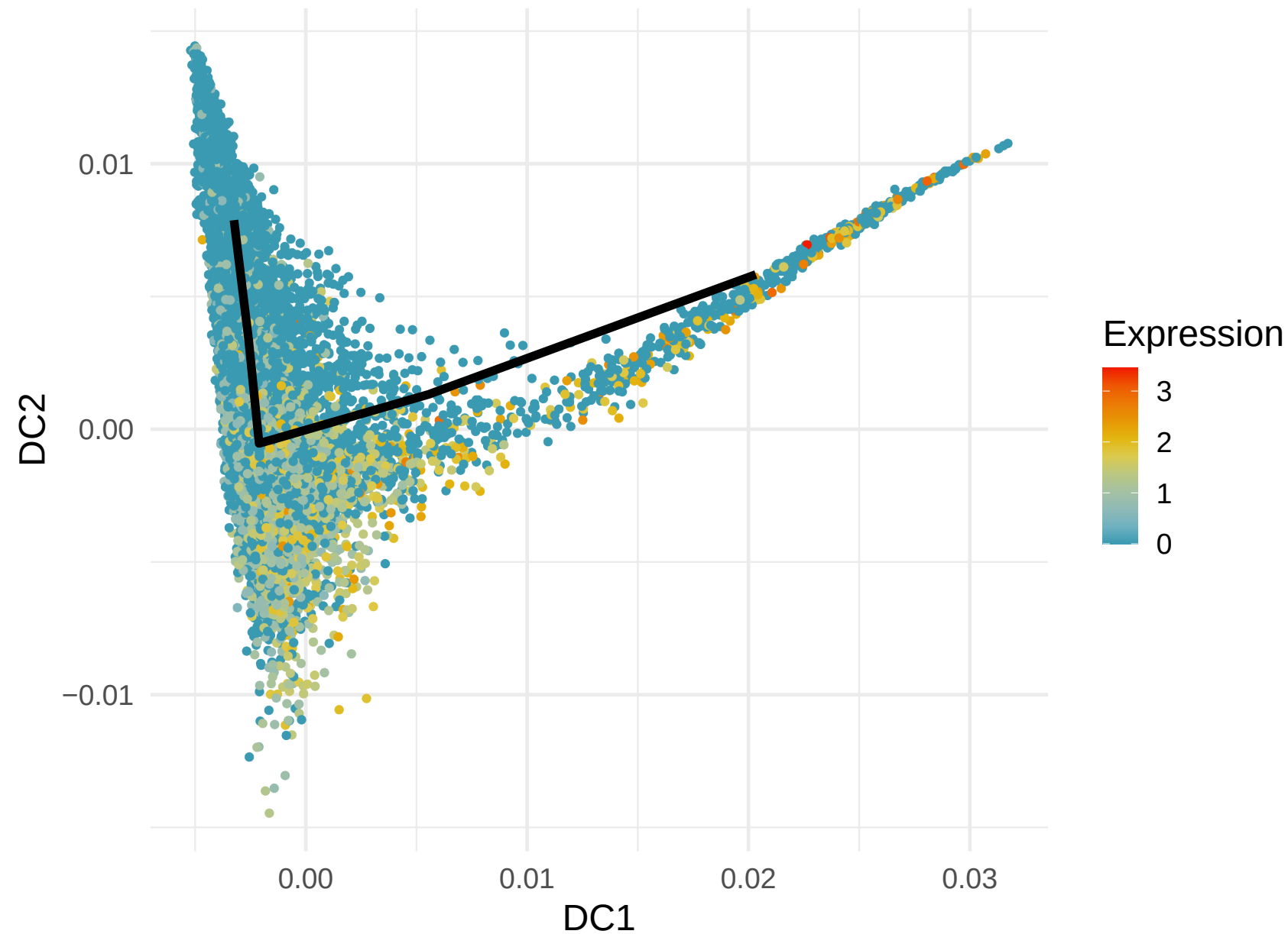
MYO1F Expression along Lineage 5 ( R = 0.269 )
