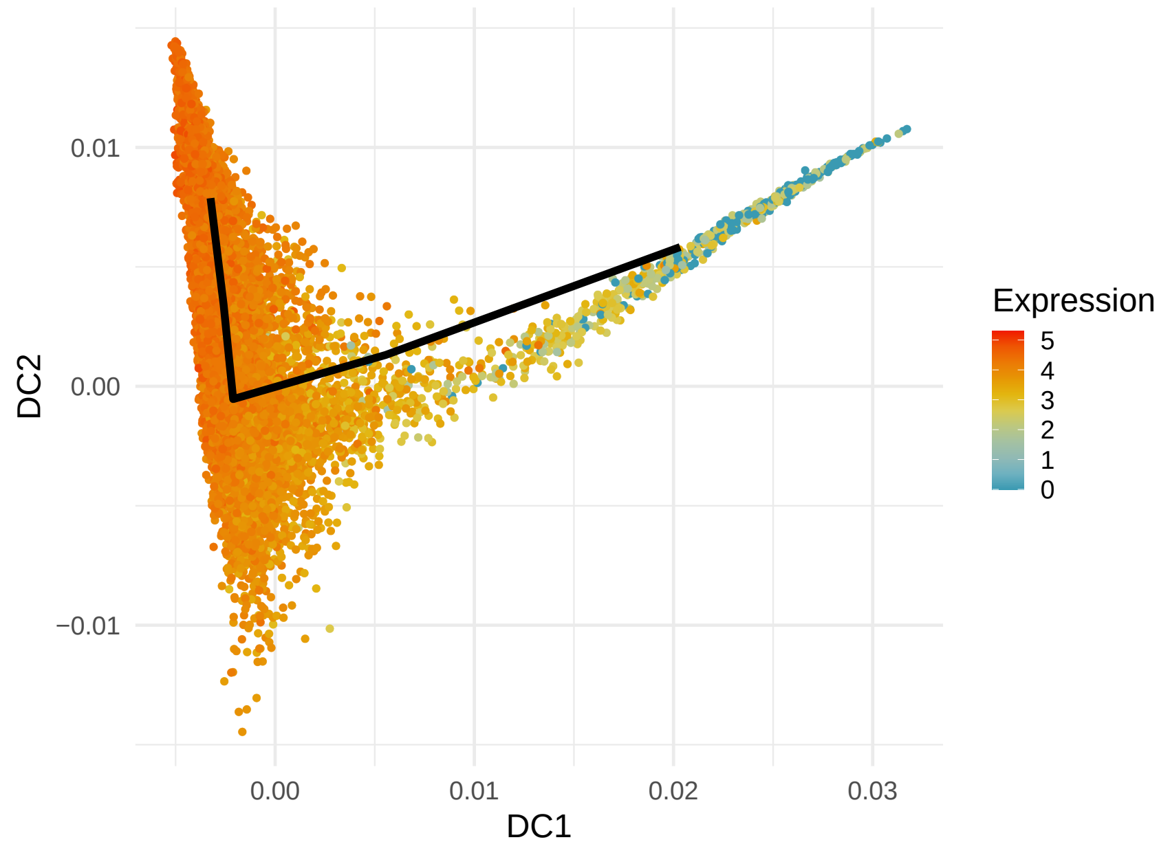
RPL11 Expression along Lineage 5 ( R = -0.567 )
