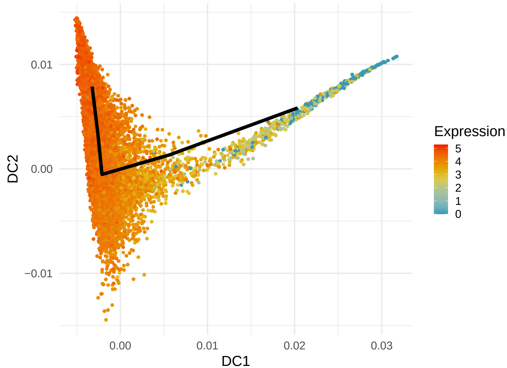
RPL30 Expression along Lineage 5 ( R = -0.597 )
