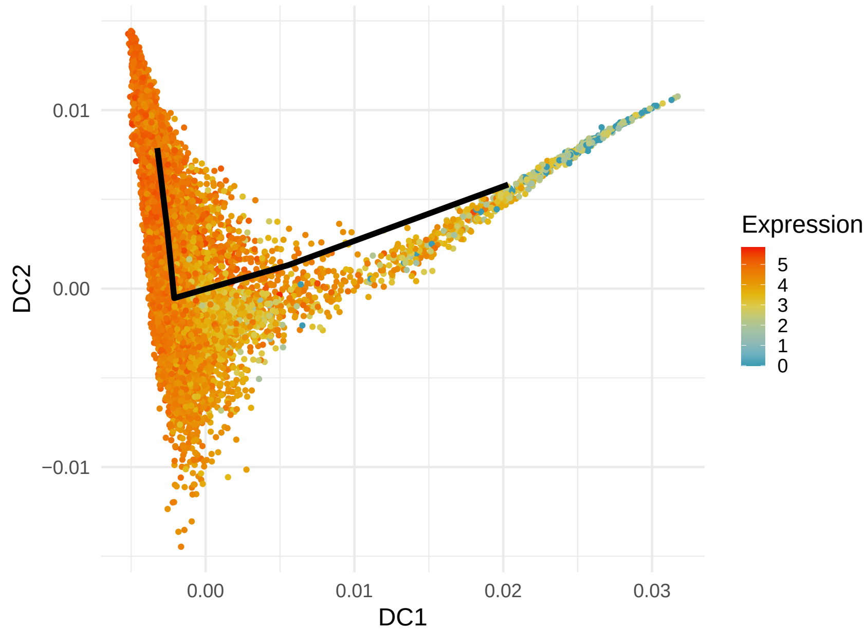
RPS27 Expression along Lineage 5 ( R = -0.559 )
