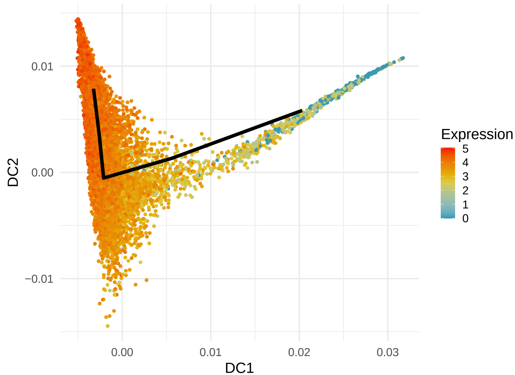
RPS3A Expression along Lineage 5 ( R = -0.589 )
