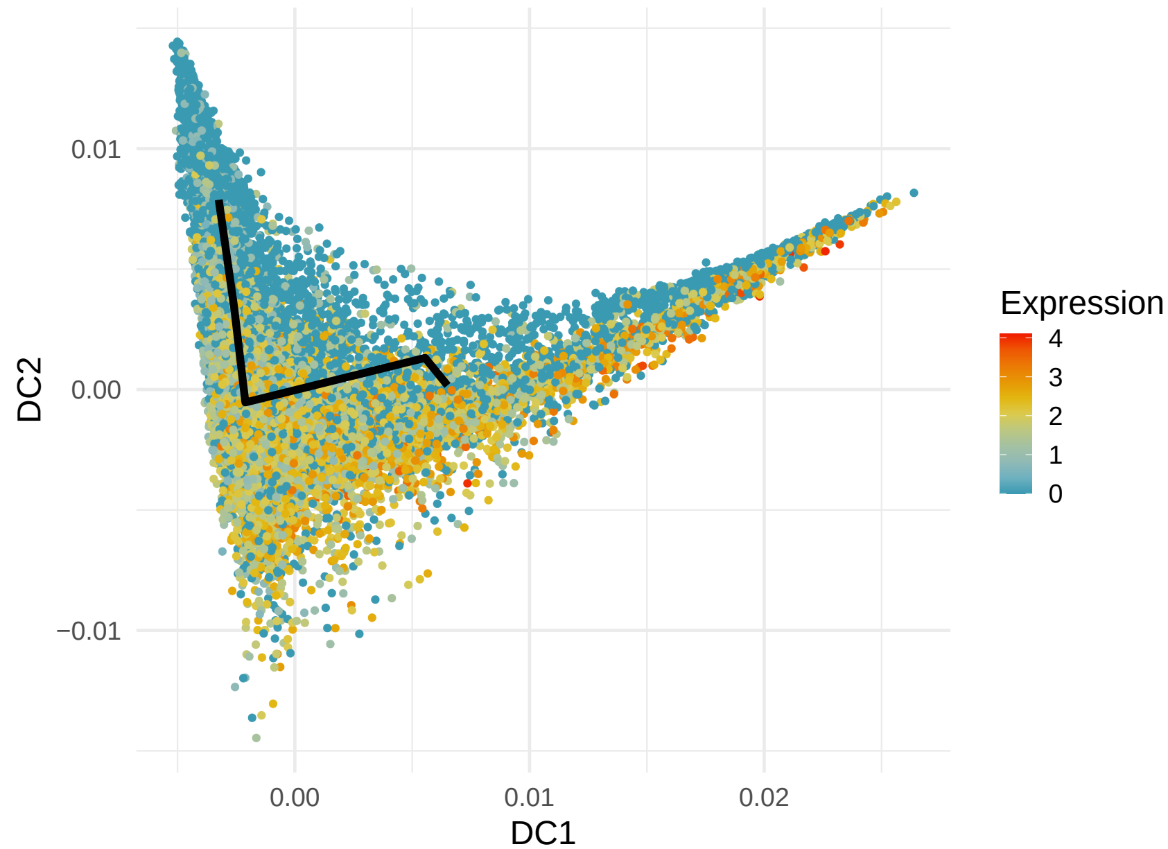
ITGB1 Expression along Lineage 6 (R= 0.348)
