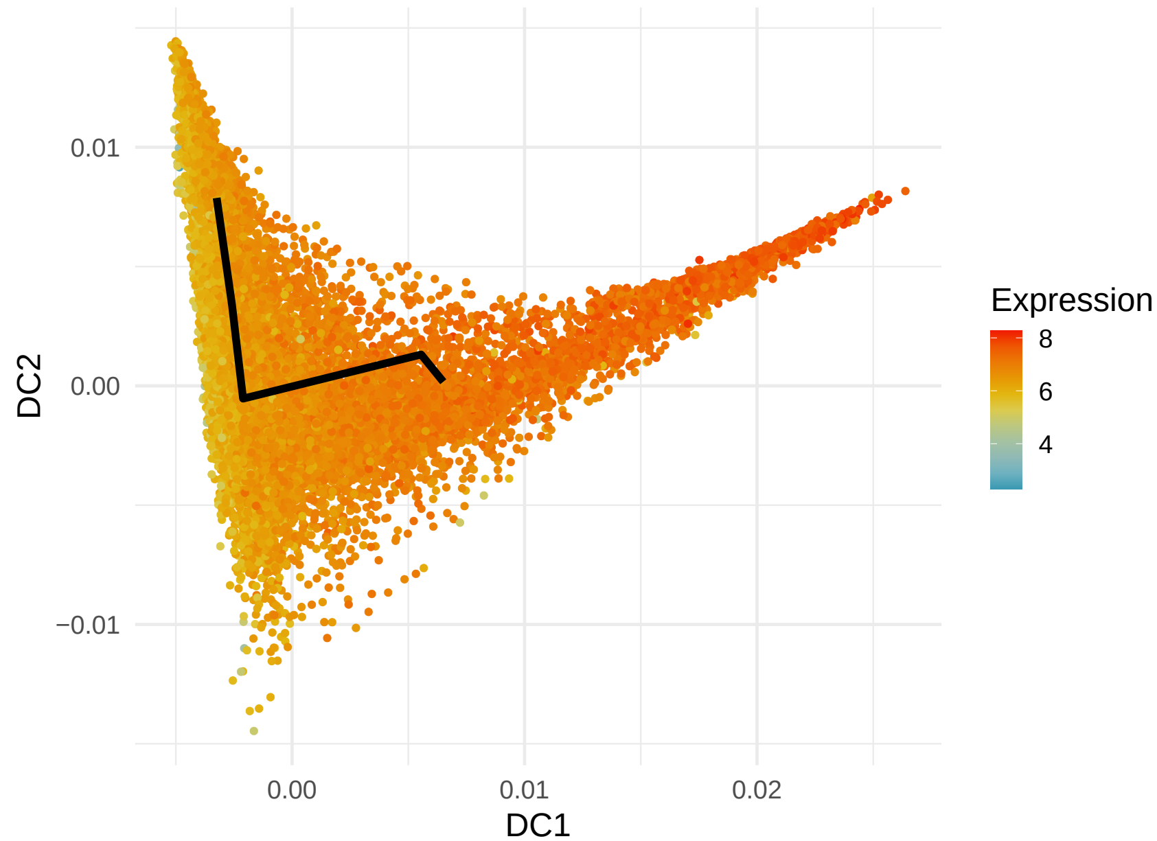
MALAT1 Expression along Lineage 6 ( R = 0.409 )
