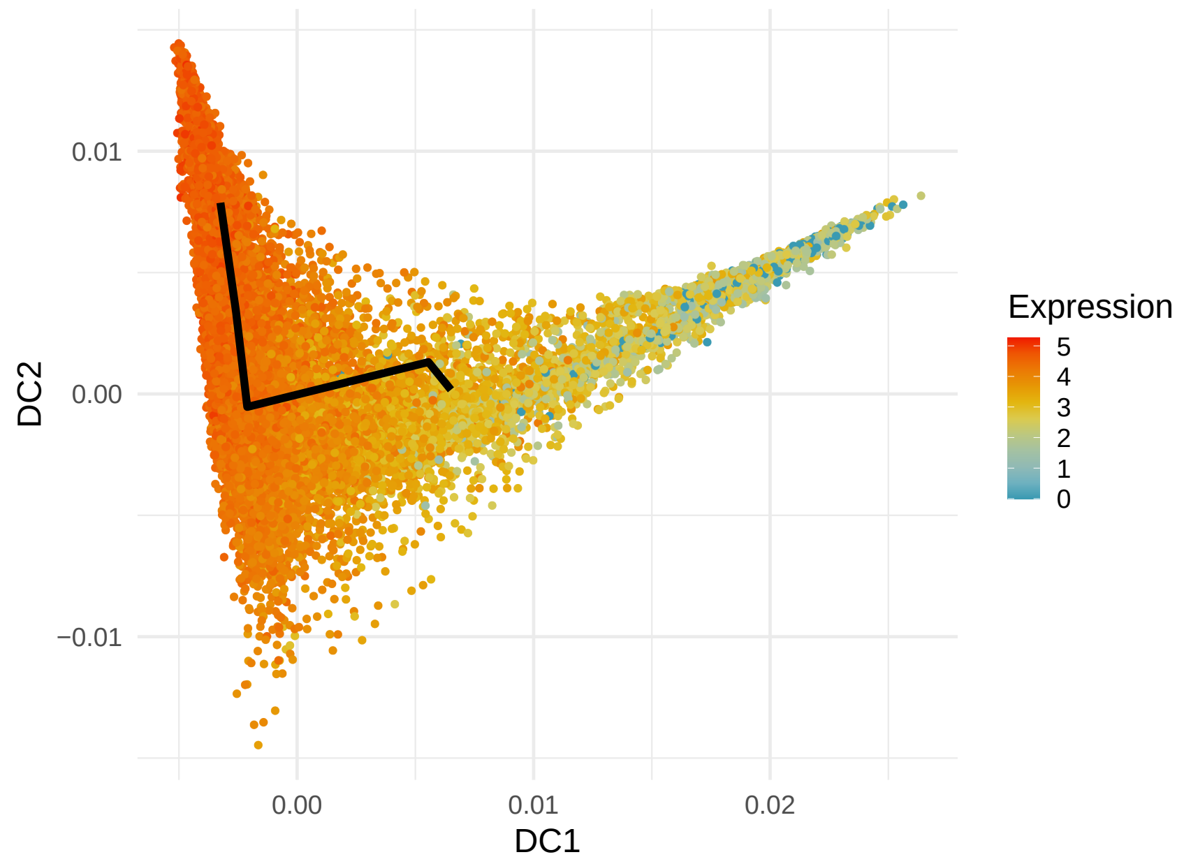
RPL30 Expression along Lineage 6 ( R = -0.555 )
