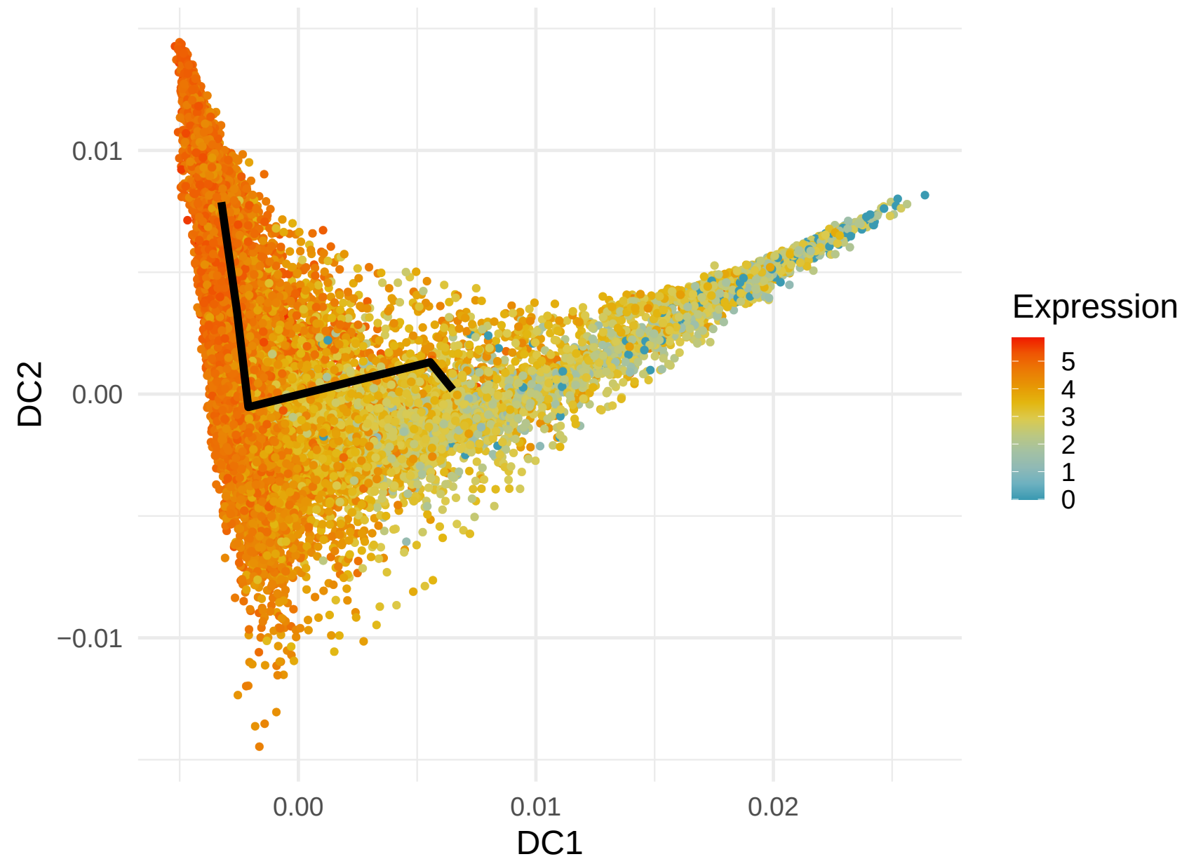
RPS27 Expression along Lineage 6 ( R = -0.603 )
