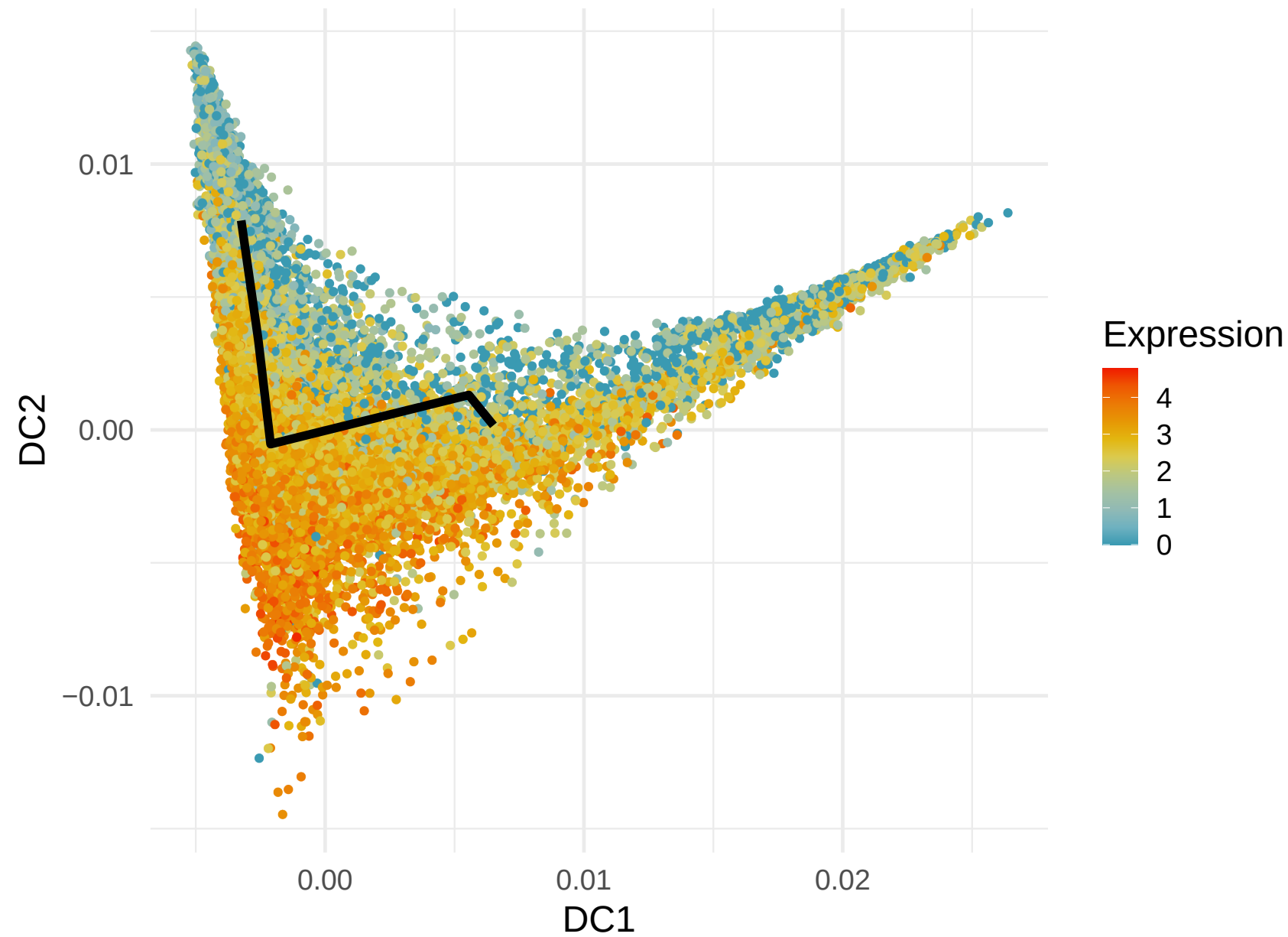
S100A4 Expression along Lineage 6 ( R = 0.346 )
