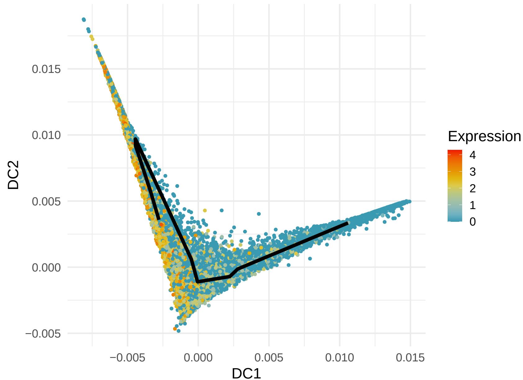
KL RD1 Expression along Lineage 1 ( R = 0.504 )
