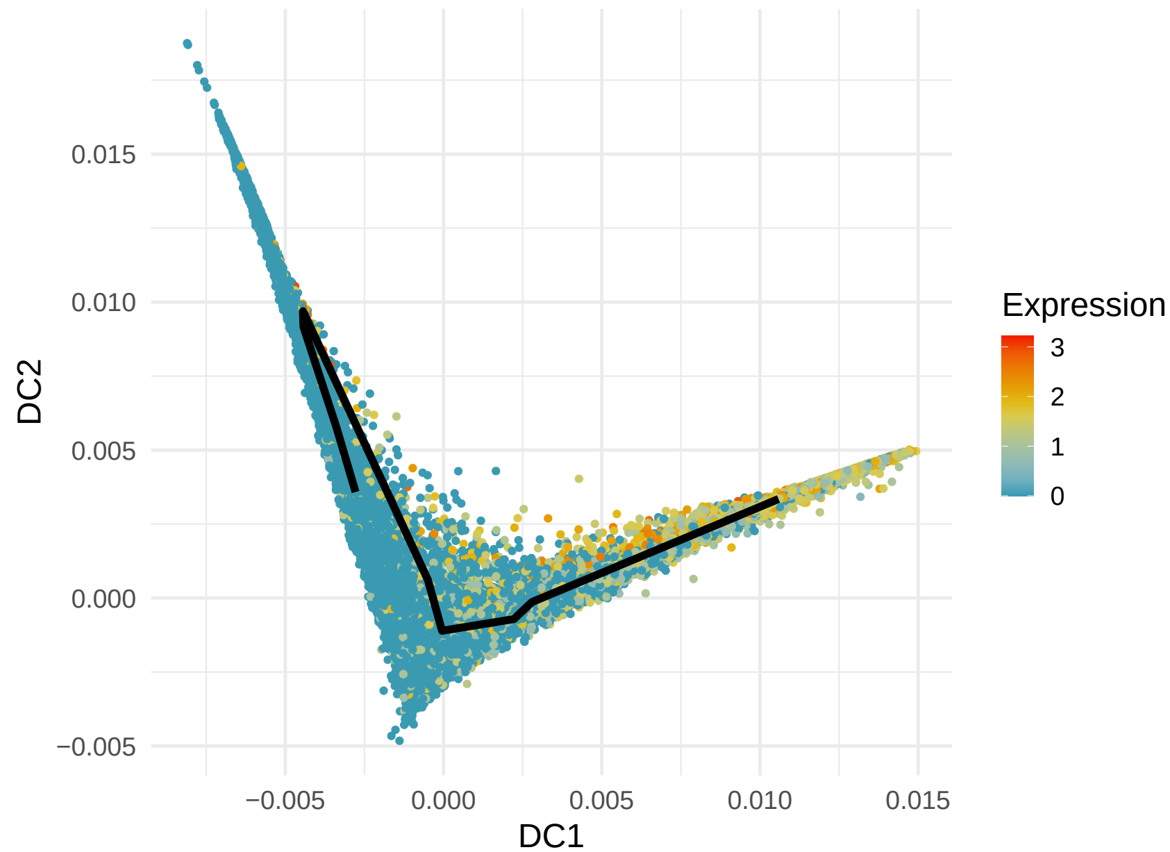
LEF1 Expression along Lineage 1 ( R = -0.557 )
