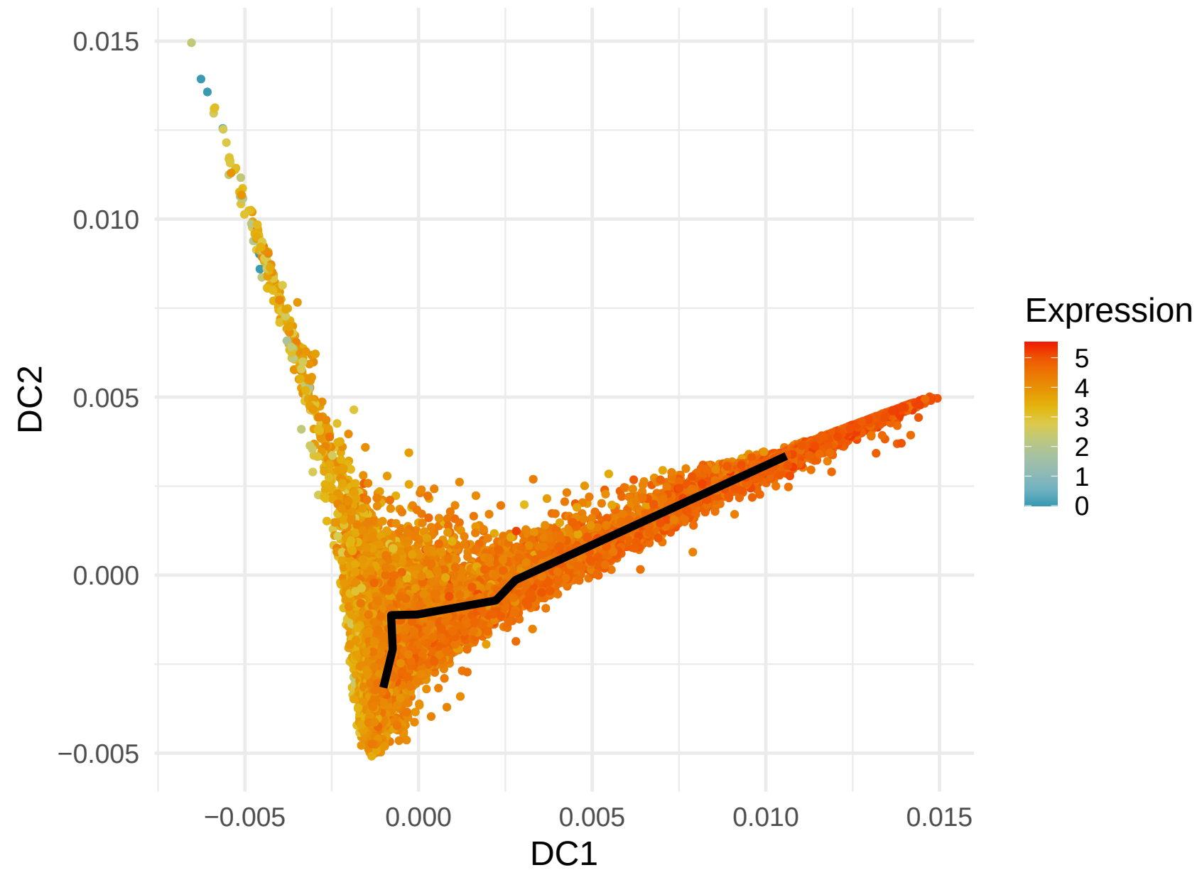
RPL13 Expression along Lineage 3 ( R = -0.604 )
