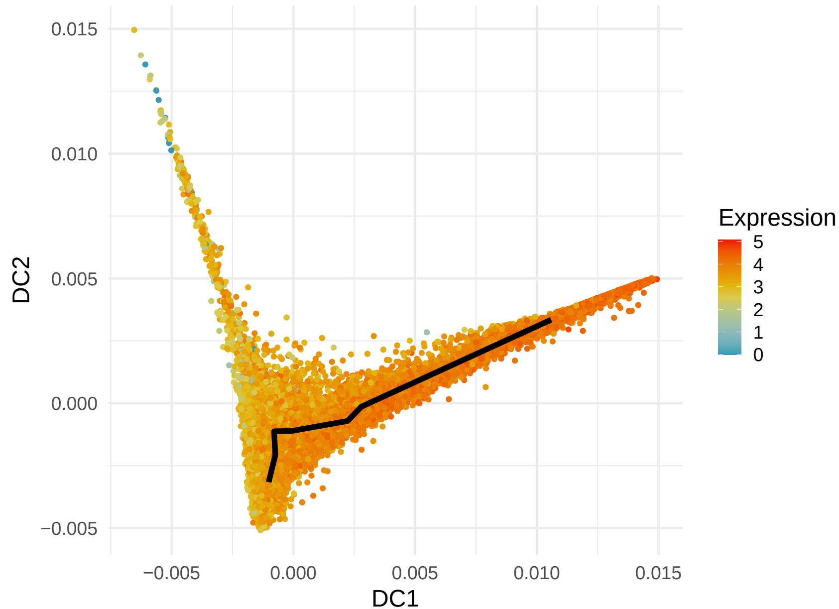
RPS28 Expression along Lineage 3 ( R = -0.534 )
