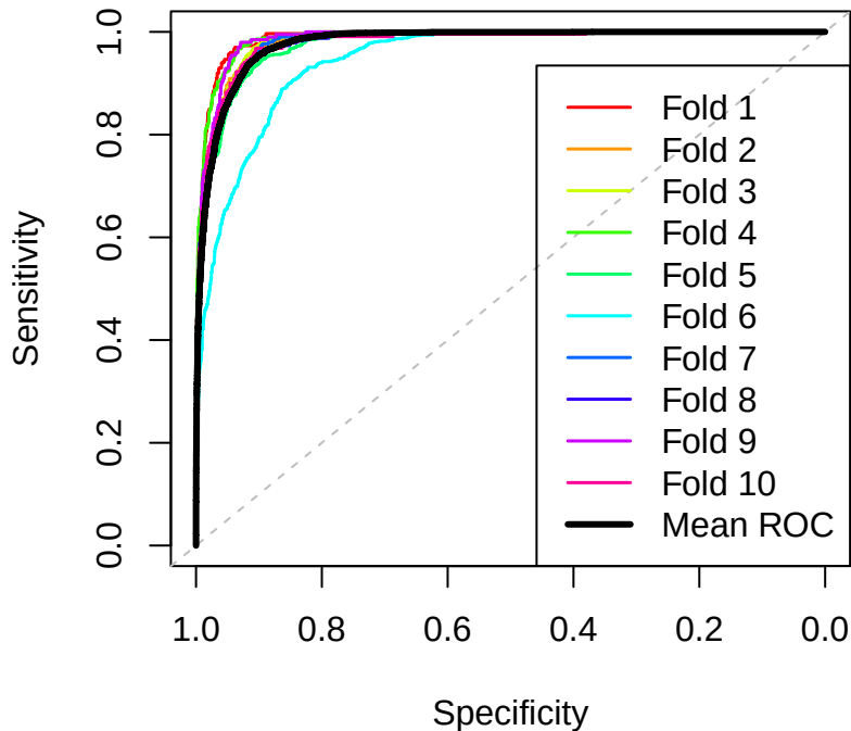
10-fold ROC Curves with Mean ROC
