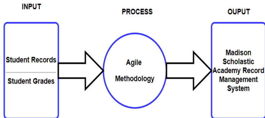
Figure 9. Input-Process-Output
