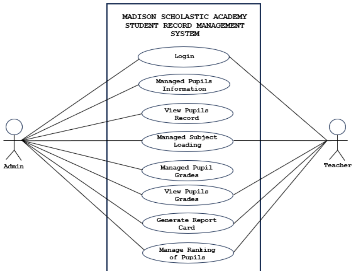
Figure 8. MSA Student Record Management System Use Case Diagram
