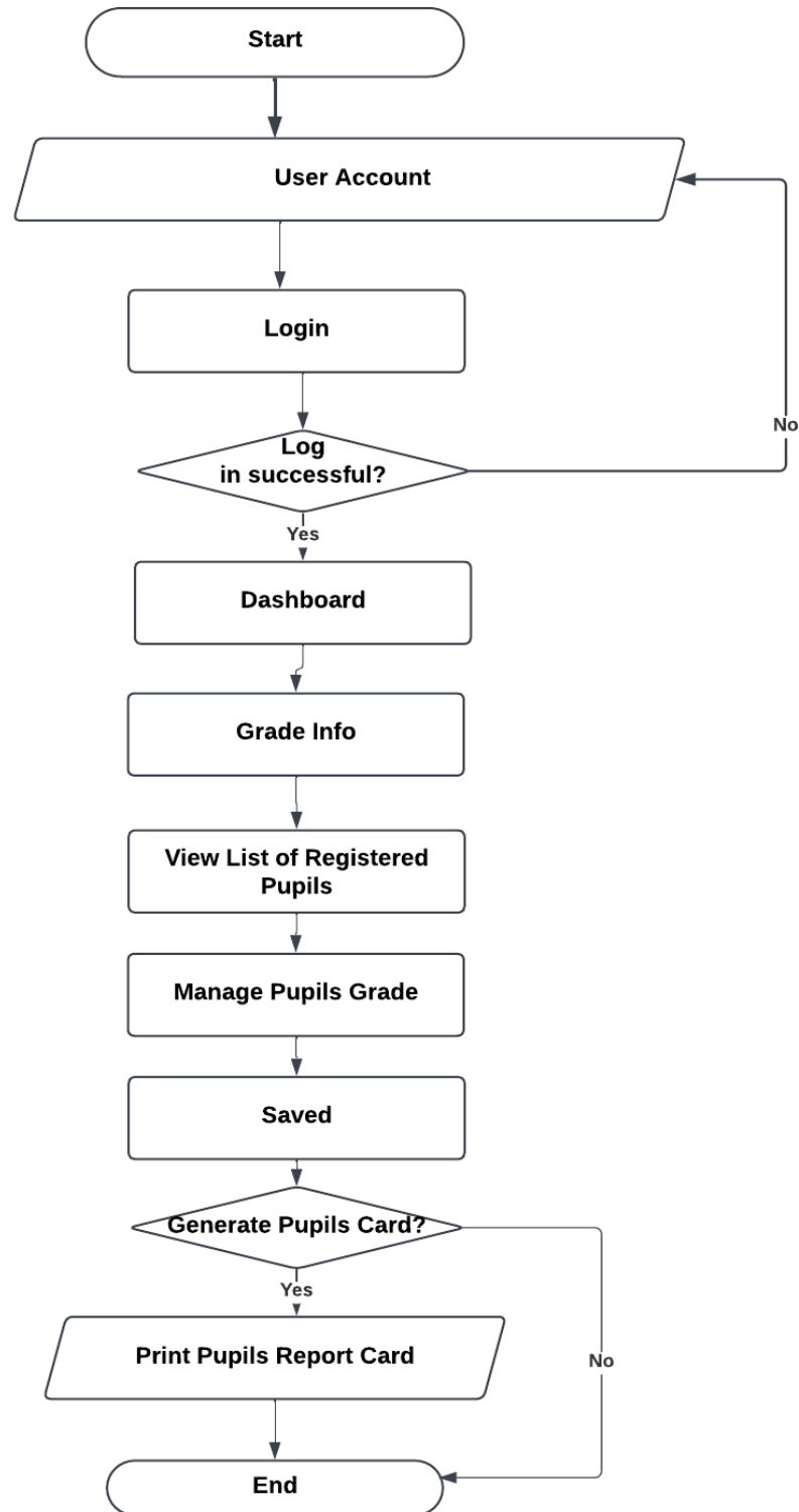
Figure 12.2. Admin/Teacher Transaction Flowchart (Grade Info)
