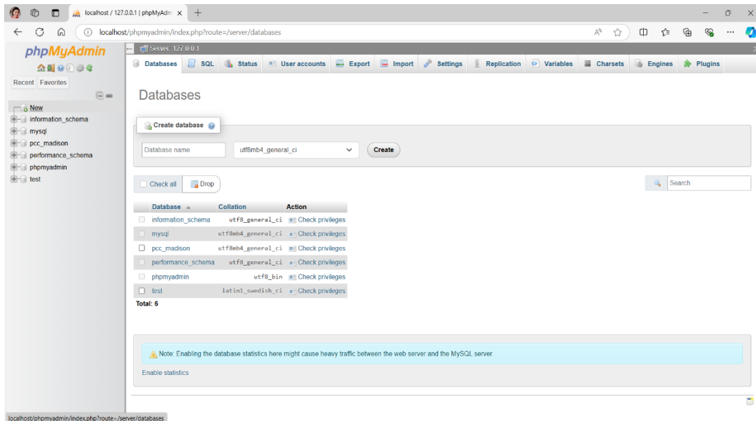
Figure 4. Creating Database
