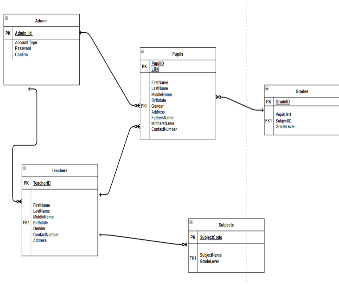
Figure 13. Entity Relationship Diagram
