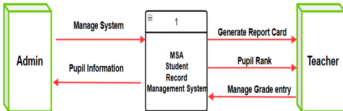
Figure 10. Context Diagram
