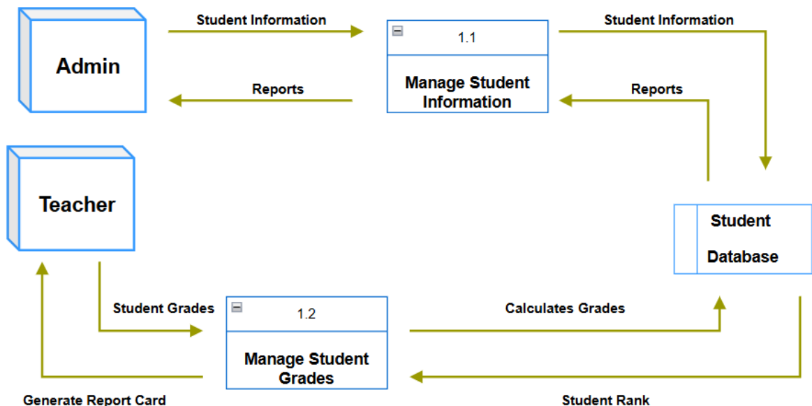
Figure 11. Data Flow Diagram (Diagram 0).
