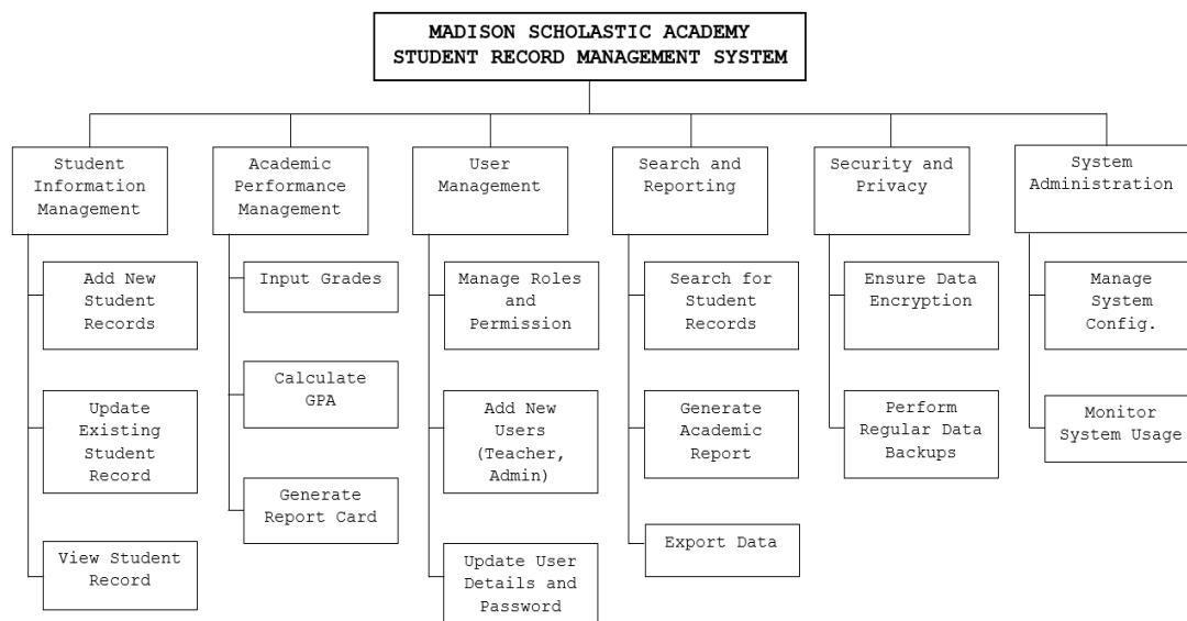
Figure 7. MSA Student Record Management System Functional Decomposition Diagram
