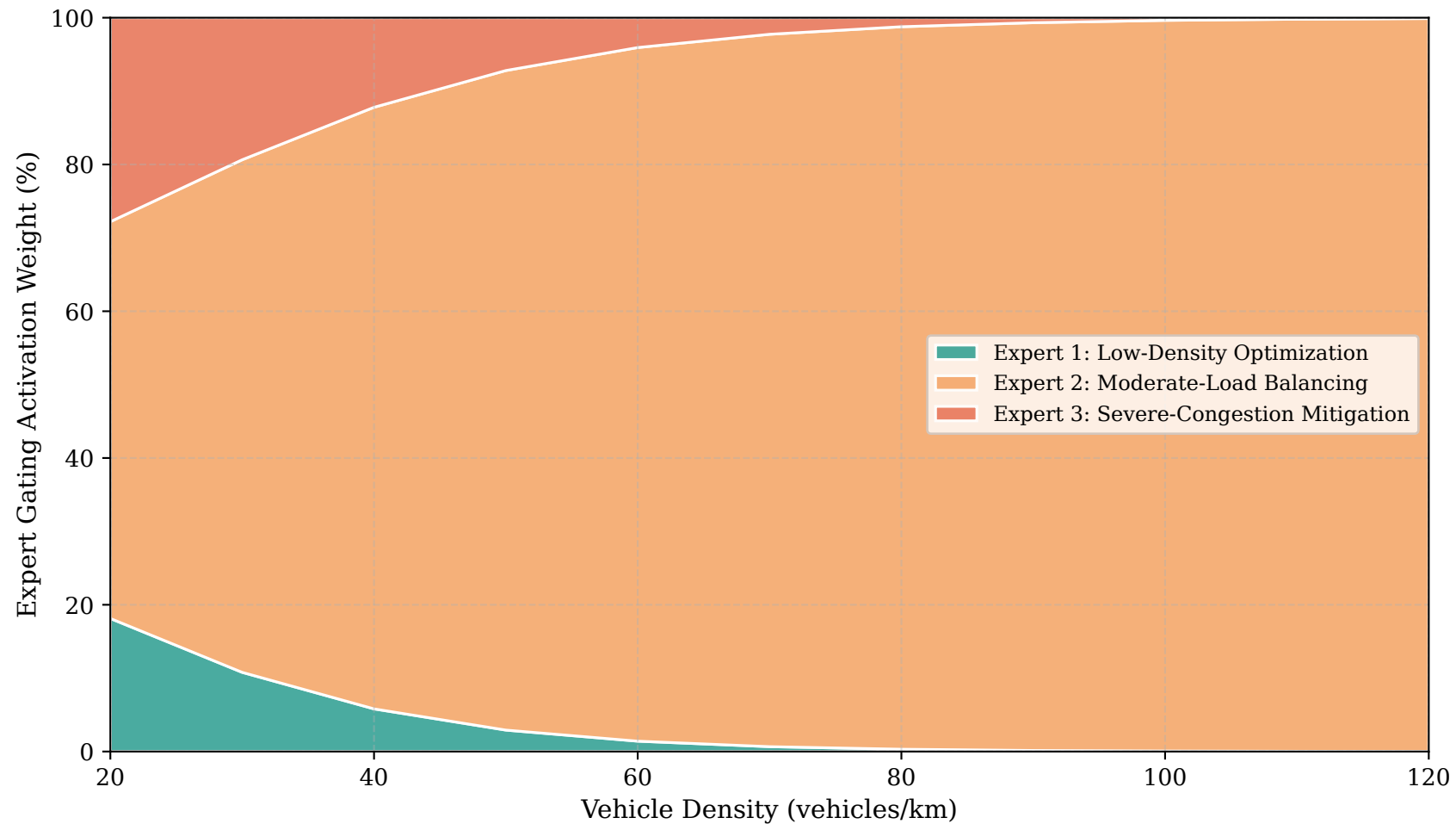
Dynamic MoE Expert Routing Weights vs. Traffic Density
