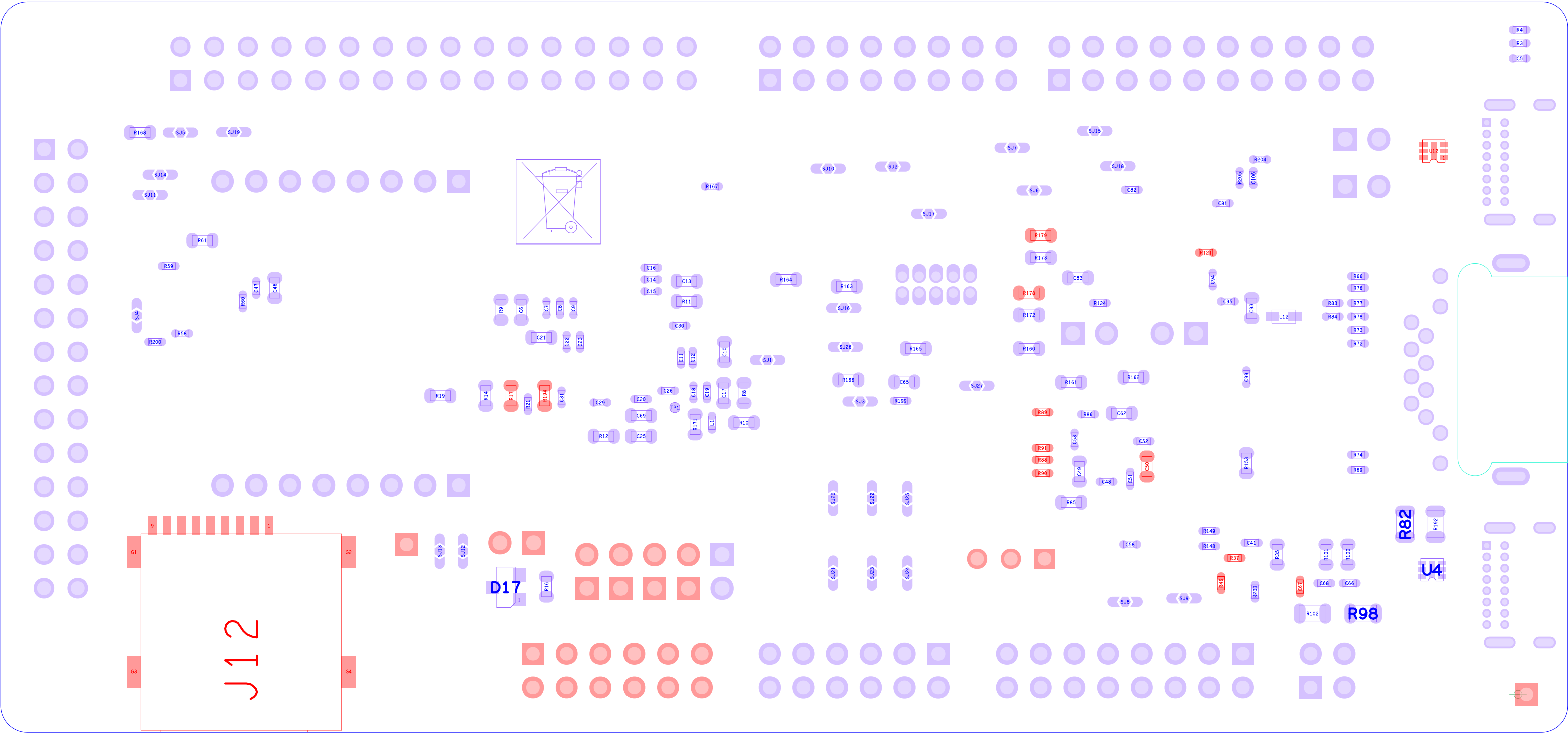
DNP - ASSY BOT TOM - LAY - 90818 REV B2 → CARD PUSH → CARD LOCK → CARD UN LOCK
