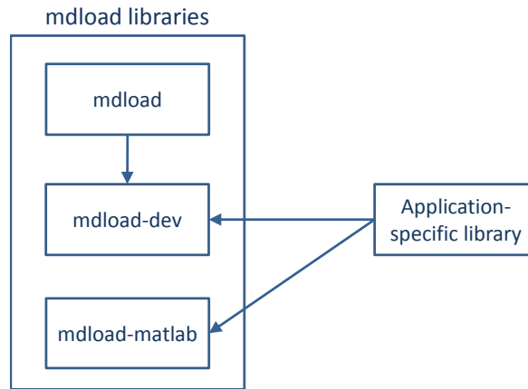
Figure 1: MDLOAD components
