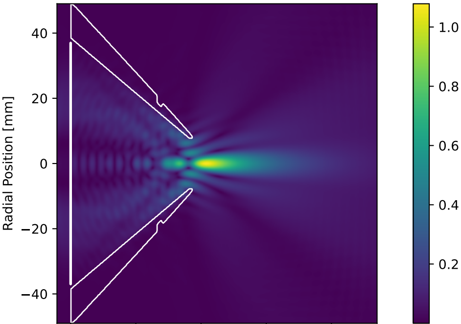
d) JAxisymmetric Steady-State Amplitude [MPa]
