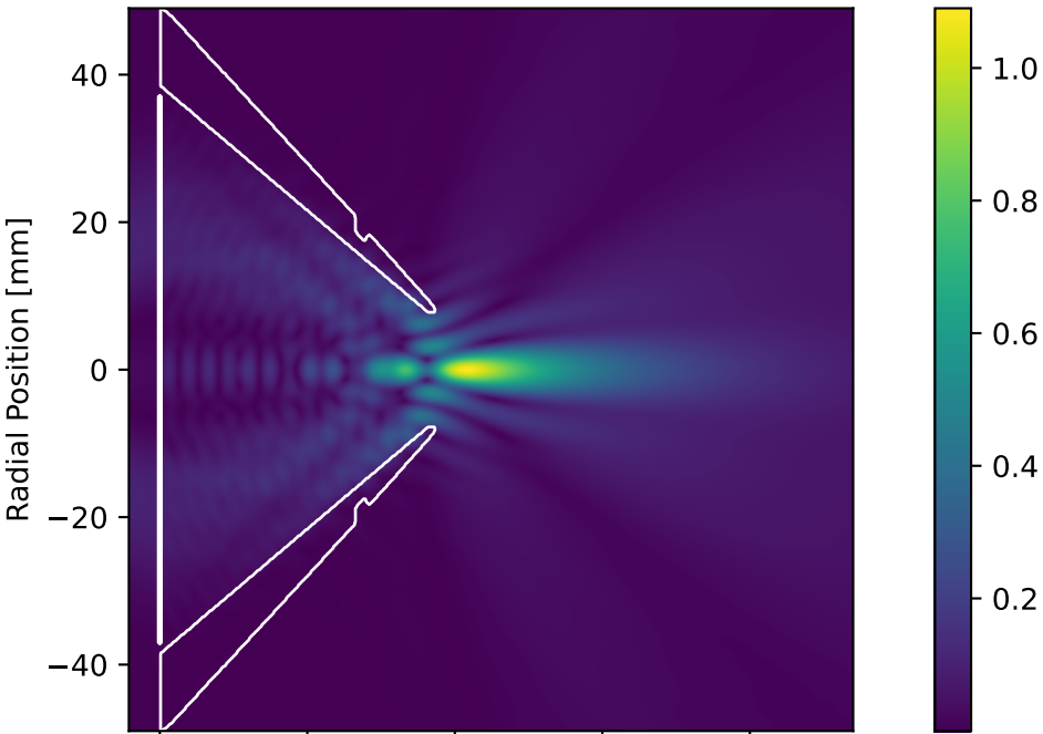
e) k-Wave Steady-State Amplitude [MPa]
