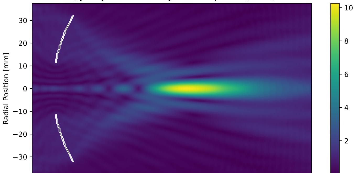
b) k-Wave Steady-State Amplitude [ref. 1]
