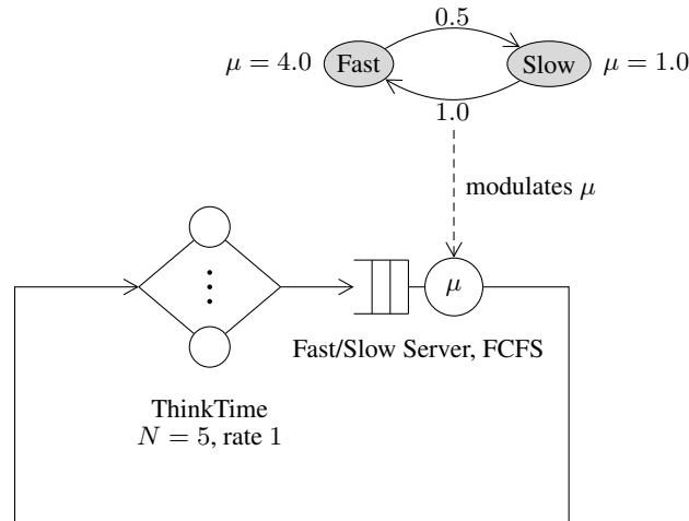
Figure 2.13: The random environment of Tutorial 12: a two-state Markov chain alternates between a fast and a slow mode, modulating the service rate of the queue in the underlying closed network.
