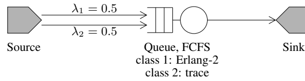
Figure 2.2: The multiclass M/G/1 queue of Tutorial 2: two open classes share one FCFS station, class 1 with Erlang-2 service and class 2 with a trace-driven service time.
