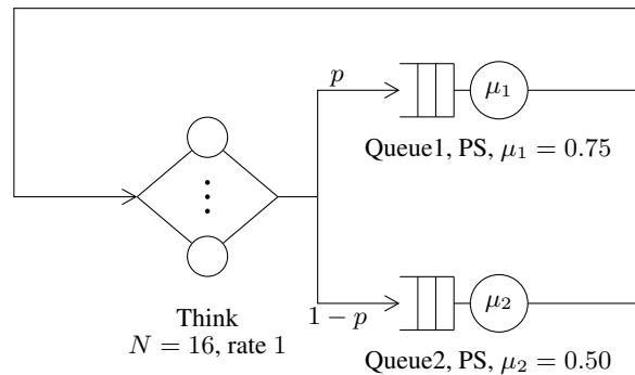
Figure 2.10: The load-balancing closed network of Tutorial 9: the routing probability p that splits the think-time output between the two queues is the decision variable of the optimization.
