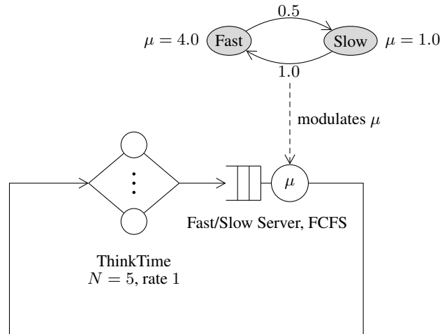
Figure 2.14: The random environment of Tutorial 12: a two-state Markov chain alternates between a fast and a slow mode, modulating the service rate of the queue in the underlying closed network.
