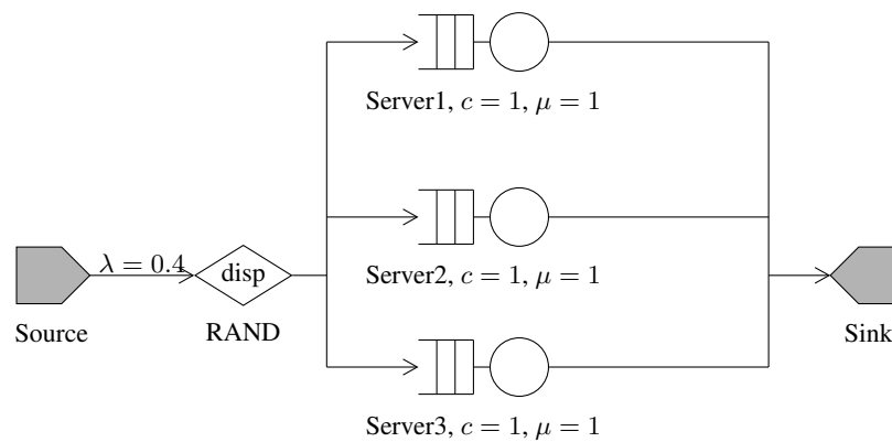
Figure 2.17: The initial open cluster of Tutorial 14: an arrival stream is dispatched at random over three single-server stations.
