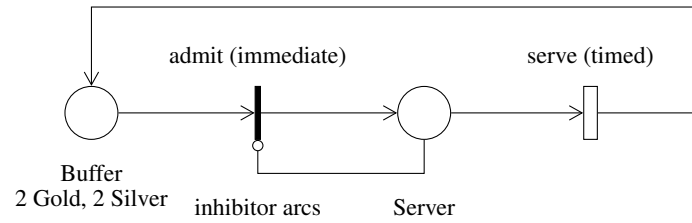
Figure 2.20: The colored GSPN of Tutorial 17. The solid thin bar is the immediate transition, the hollow bar the timed one, and the arc ending in a small circle is the inhibitor pair that keeps the server to one token: each of admit 's two modes is inhibited by a token of either color in Server .
