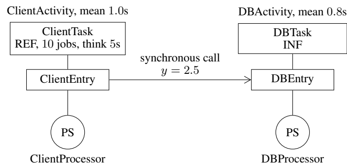
Figure 2.13: The layered network of Tutorial 11: the client task issues on average 2.5 synchronous calls per request to the database entry, and each task runs on its own processor.
