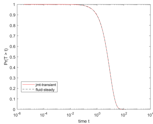
Figure 2.9: Comparison of simulated response time distribution and its fluid approximation
