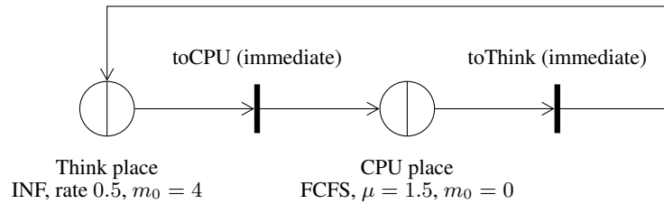
Figure 2.19: The queueing Petri net of Tutorial 16: two queueing places, drawn in the standard queueing-Petri-net shorthand as a place circle bisected by a vertical bar, exchange a single token per firing of the immediate transitions. The bar stands for the scheduling station embedded in the place, whose completions reach the depository from which the output transition consumes them; an ordinary place would be an undivided circle.
