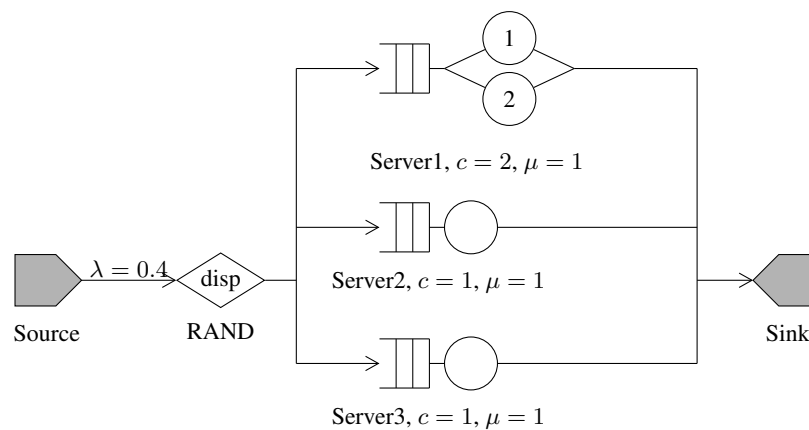
Figure 2.17: The open cluster of Tutorial 14: an arrival stream is dispatched at random over three stations, the first of which has two servers.
