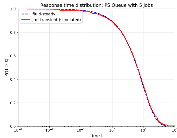
Figure 2.9: Comparison of simulated response time distribution and its fluid approximation
