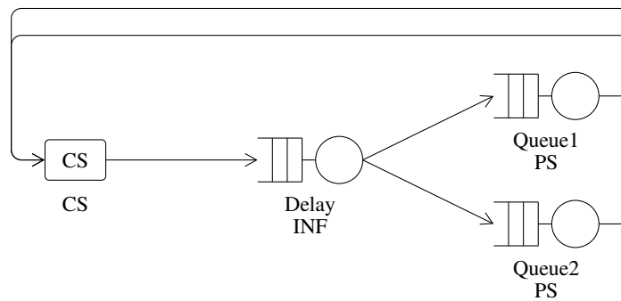
Figure 2.20: Topology of cqn_twoclass_erl : a closed network over 3 queueing stations with a class-switch node.
