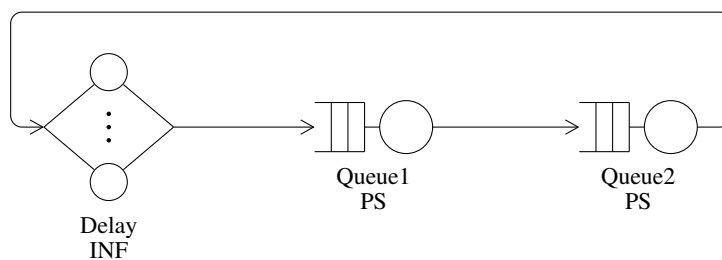
Figure 3.24: Topology of statepr_sys_marg: a closed network over 3 queueing stations.
