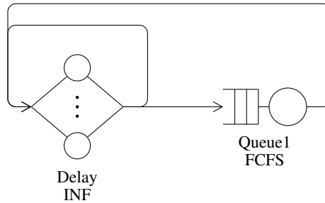
Figure 2.16: Topology of cqn_repairmen: a closed network over 2 queuing stations.
