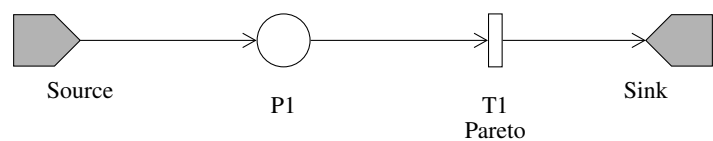
Figure 2.98: Topology of spn_pareto_service : a stochastic Petri net over 1 place and 1 transition; a place is a circle holding its initial marking and a transition a bar, hollow when its firing time is random and solid when it fires at once; the net is open, fed by a Source and drained into a Sink.
