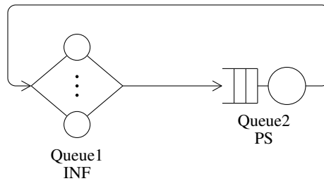
Figure 3.53: Topology of renv_twestages_repairmen : a closed network over 2 queueing stations.
