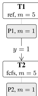
Figure 2.66: Call graph of lqn_transient: 2 tasks over 2 processors, drawn with the reference task on top and a called task below its caller; the shaded box under each task is the processor it runs on.
