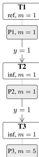
Figure 2.68: Call graph of lqn_workflows: 3 tasks over 3 processors, drawn with the reference task on top and a called task below its caller; the shaded box under each task is the processor it runs on.
