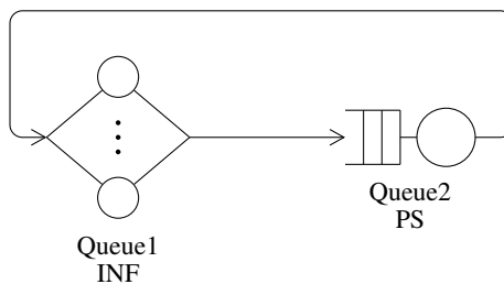
Figure 3.50: Topology of renv_genqn : a closed network over 2 queueing stations.
