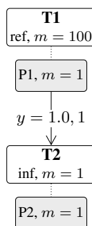
Figure 2.59: Call graph of lqn_moment3: 2 tasks over 2 processors, drawn with the reference task on top and a called task below its caller; the shaded box under each task is the processor it runs on.
