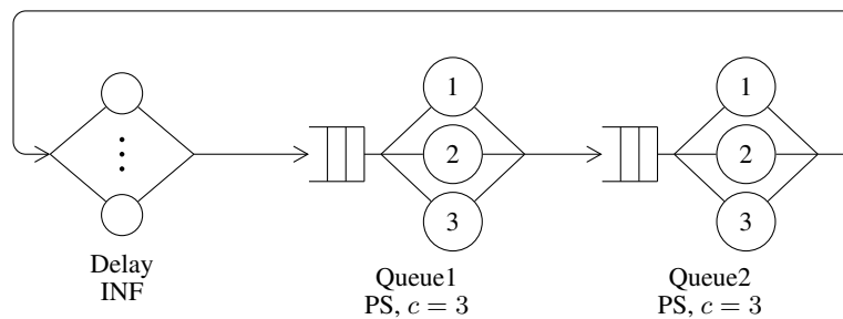
Figure 3.9: Topology of ld_multiserver_ps : a closed network over 3 queueing stations.
