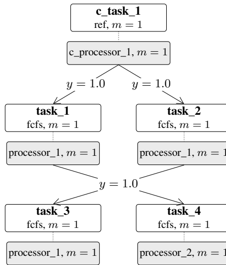
Figure 4.30: Call graph of gallery_lqn_random: 5 tasks over 3 processors, drawn with the reference task on top and a called task below its caller; the shaded box under each task is the processor it runs on.
