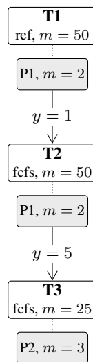
Figure 4.29: Call graph of gallery_lqn_basic: 3 tasks over 2 processors, drawn with the reference task on top and a called task below its caller; the shaded box under each task is the processor it runs on.
