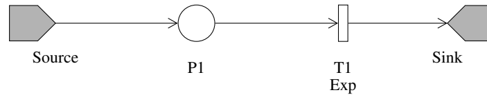
Figure 2.91: Topology of spn_basic_open : a stochastic Petri net over 1 place and 1 transition; a place is a circle holding its initial marking and a transition a bar, hollow when its firing time is random and solid when it fires at once; the net is open, fed by a Source and drained into a Sink.
