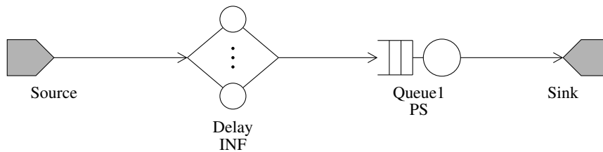
Figure 8.5: Topology of est_erps_open : an open network over 2 queueing stations.
