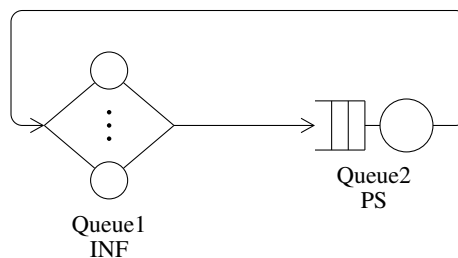
Figure 3.49: Topology of renv_fourstages_repairmen : a closed network over 2 queueing stations.
