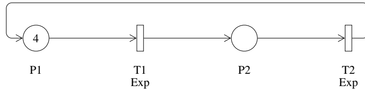
Figure 2.94: Topology of spn_fluid_dae : a stochastic Petri net over 2 places and 2 transitions; a place is a circle holding its initial marking and a transition a bar, hollow when its firing time is random and solid when it fires at once.
