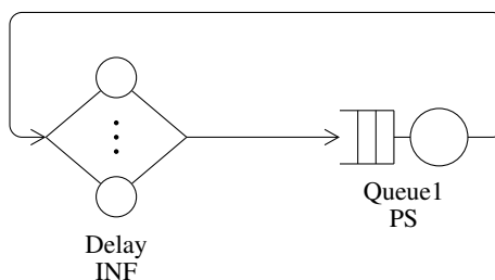
Figure 8.12: Topology of est_ubo_variants_closed: a closed network over 2 queueing stations.
