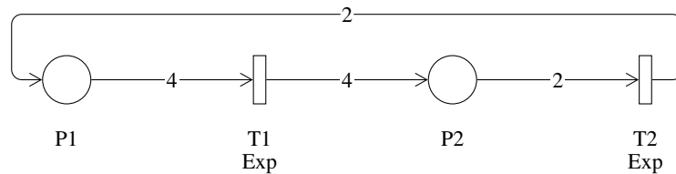
Figure 2.100: Topology of spn_twomodes: a stochastic Petri net over 2 places and 2 transitions; a place is a circle holding its initial marking and a transition a bar, hollow when its firing time is random and solid when it fires at once; an arc that moves more than one token carries its multiplicity.
