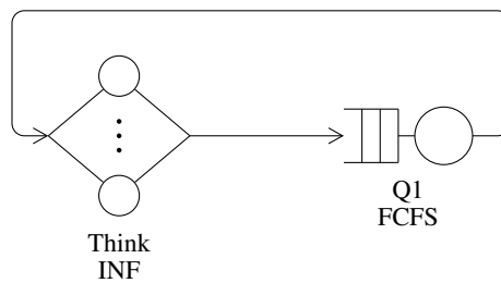
Figure 3.51: Topology of renv_map_fallback: a closed network over 2 queueing stations.
