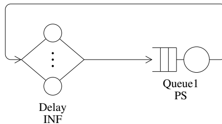
Figure 8.10: Topology of est_ubo_closed: a closed network over 2 queueing stations.
