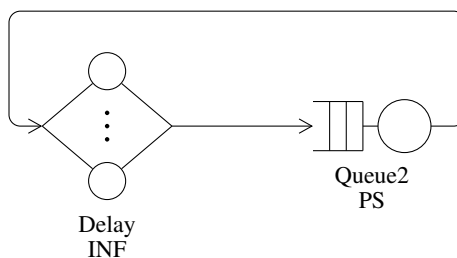
Figure 3.39: Topology of cdf_respt_closed : a closed network over 2 queueing stations.
