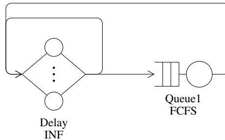
Figure 2.16: Topology of cqn_repairmen: a closed network over 2 queueing stations.
