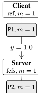
Figure 2.58: Call graph of lqn_fork_open_arrival: 2 tasks over 2 processors, drawn with the reference task on top and a called task below its caller; the shaded box under each task is the processor it runs on.
