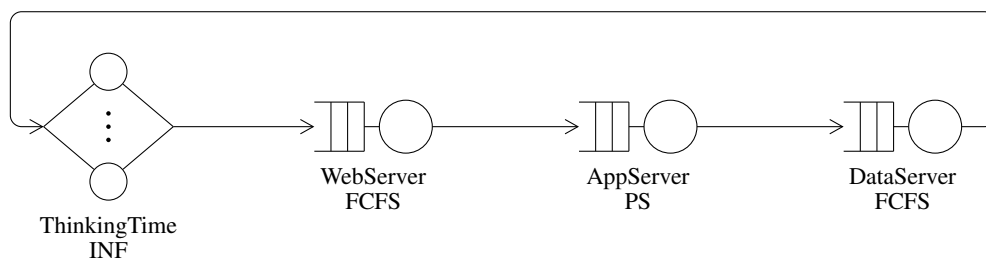
Figure 2.12: Topology of cqn_multichain_cs: a closed network over 4 queuing stations.
